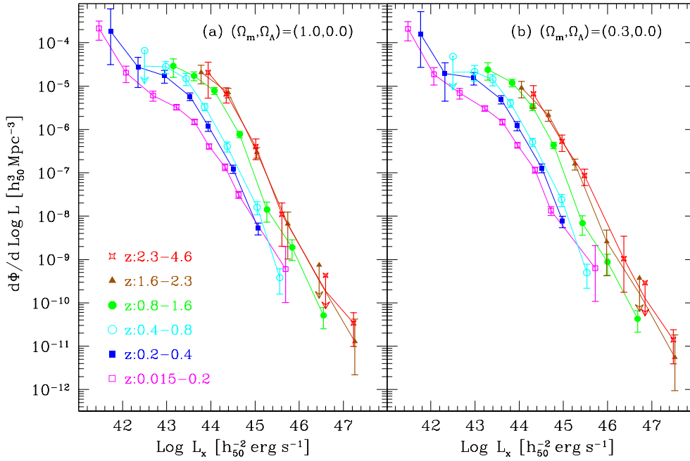
Fig. 3a and b. The \Sigma V_a^{-1} estimates of the SXLFs are plotted with estimated 1\sigma errors. Different symbols correspond to different redshift bins as indicated in the panel a and data points belonging to the same redshift bin are connected. The position of the symbol attached to a downward arrow indicates the 90% upper limit (corresponding to 2.3 objects), where there is no AGN detected in the bin.
