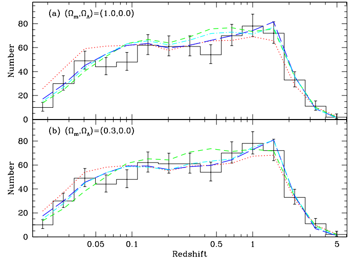
Fig. 7. The redshift distribution of the AGN sample, histogrammed in equal interval in \log z , is compared with predictions from the best-fit PLE (dotted), PDE (shot-dashed), LDDE1 (long-dashed), and LDDE2 (dot-dashed) models for two sets of cosmological parameters as labeled. The asymmetric error bars correspond to approximate 1\sigma Poisson errors calculated using Eqs. (7) and (11) of Gehrels (1986) with S = 1 .
