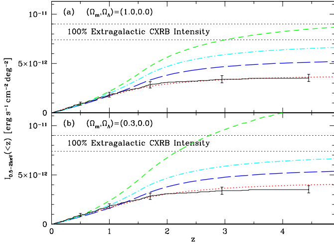
Fig. 10. The cumulative 0.5–2 keV intensities I(< z) are plotted as a function of redshift for the PLE, PDE, LDDE1, and LDDE2 models for two different cosmologies as labeled. See caption for Fig. 5 for line styles corresponding to these four models. These curves include expected contribution from sources fainter than the survey limit using the model extrapolations. As a reference, the cumulative intensity I(< z) of the AGNs in the sample (see text) is also plotted (thin solid line with 90% errors) on each panel. This curve represents the contribution of actually resolved and identified AGNs. Also the range of the 0.5–2 keV extragalactic background intensity (see text) is shown by two horizontal thin dotted lines.
