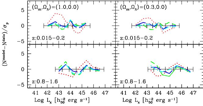
Fig. 9. Residuals in the -\chi space (see text) are shown for two redshift bins, i.e., 0.015 \leq z < 0.2 and 0.8 \leq z < 1.6 , where differences among different models are apparent. Different line styles correspond to different models. See caption for Fig. 5 for the line styles. The luminosity bins are shown as horizontal bars bordered by ticks.
