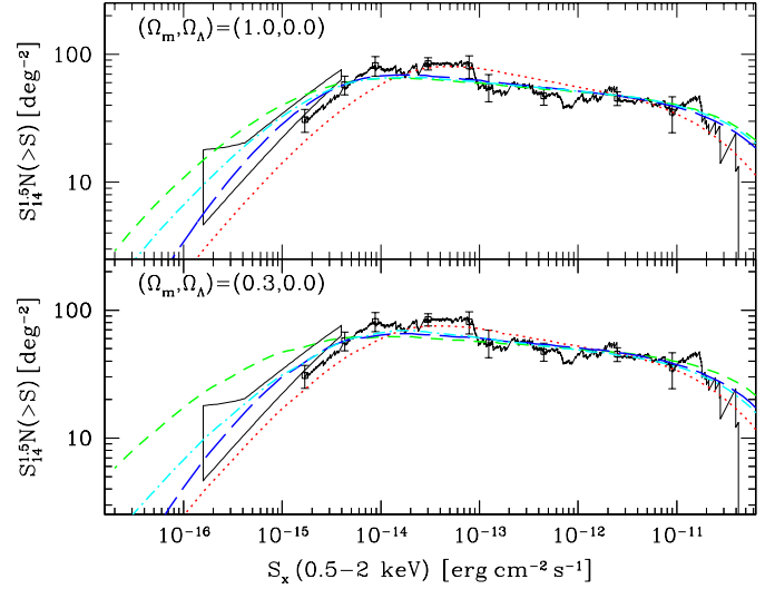
Fig. 6. The S^{1.5} N(>S) (a horizontal line corresponds to the Euclidean slope) curve for our sample AGNs is plotted with 90% errors at several locations and are compared with the best-fit PLE (dotted), PDE (shot-dashed), LDDE1 (long-dashed), LDDE2 (dot-dashed) models for the (\Omega_m, \Omega_\Lambda) = (1, 0) (upper panel) and (0.3, 0) (lower panel). The thin-solid fish is from the fluctuation analysis of the Lockman Hole HRI data (including non-AGNs) by Hasinger et al. (1993)
