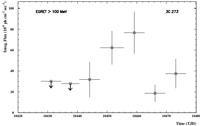
Fig. 2. The EGRET light curve of 3C 273 at energy above 100 MeV for the seven individual VPs (for the calendar dates see Table 1). The quasar was not detected during the beginning of the observations, then showed a flux increase to the highest level ever for \sim 2 weeks in the middle part (VPs 609 and 610), and then returned to about the previous flux level in the last two weeks. The errors are 1\sigma and the upper limits are 2\sigma .
