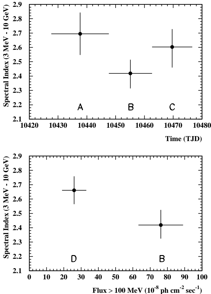
Fig. 7. The spectral index (3 MeV - 10 GeV) as a function of time (periods A, B, and C) is shown in the upper panel and of source flux > 100 MeV (periods B and D (A+C)) in the lower panel. The errors are 1\sigma . There is evidence for spectral hardening with increasing flux.
