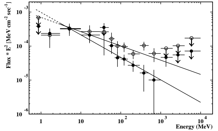
Fig. 6. The spectra of the flare state (B, open circles) and the sum of the lower flux levels (A+C, filled circles) are compared. The two spectra differ mainly above 100 MeV.
