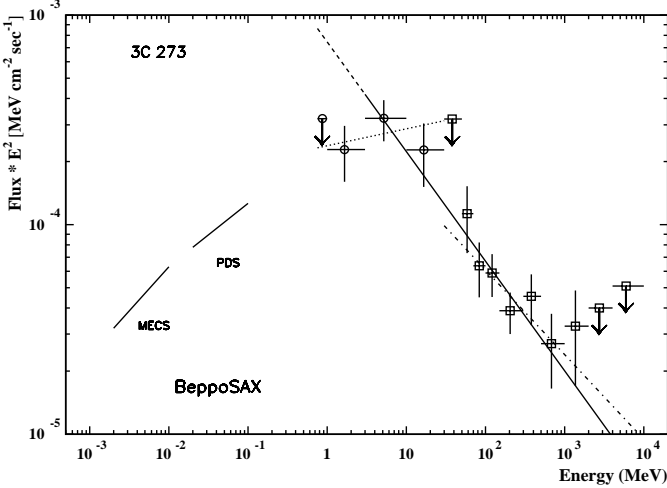
Fig. 4. Quasi-simultaneous BeppoSAX-CGRO high-energy spectrum of 3C 273 in an E^2 \times differential-flux representation. The EGRET ( \square ) and COMPTEL ( \circ ) spectral points are derived from the sum of the whole observation (7 weeks). The errors are 1\sigma and the upper limits are 2\sigma . An upper limit is drawn when the significance of an individual flux value is less than 1\sigma . The solid line represents the best-fit power-law model for the range 3 MeV to 10 GeV. The dashed line shows the extrapolation towards lower energies. The dotted line represents the best-fit power-law model for only the COMPTEL data (0.75-30 MeV) and the dashed-dotted line the one for solely the EGRET data (30 MeV - 10 GeV). The BeppoSAX power-law shapes were observed on January 13, 1999 (Haardt et al. 1998), located within the CGRO observational period. The strong spectral turnover at a few MeV is evident.
