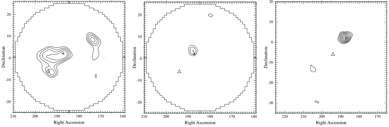
Fig. 1. Virgo maps in the \gamma -ray energy bands 3-10 MeV (left), 10-30 MeV (middle) as observed by COMPTEL, and >100 MeV (right) as provided by EGRET for the complete set of 7 weeks of continuous data (VPs 606 to 611.1). For COMPTEL the contour lines start at a detection significance of 3\sigma ( \chi^2_1 -statistics for a known source) with a step of 0.5\sigma . For EGRET the contour lines also start at a detection significance of 3\sigma , however with a step of 1\sigma . The locations of the famous Virgo blazars 3C 273 (+) and 3C 279 ( \Delta ) are indicated. 3C 273 is detected with 10.4\sigma by EGRET. There is significant emission from 3C 273 in both COMPTEL maps. The COMPTEL 3-10 MeV map shows hints for additional sources.
