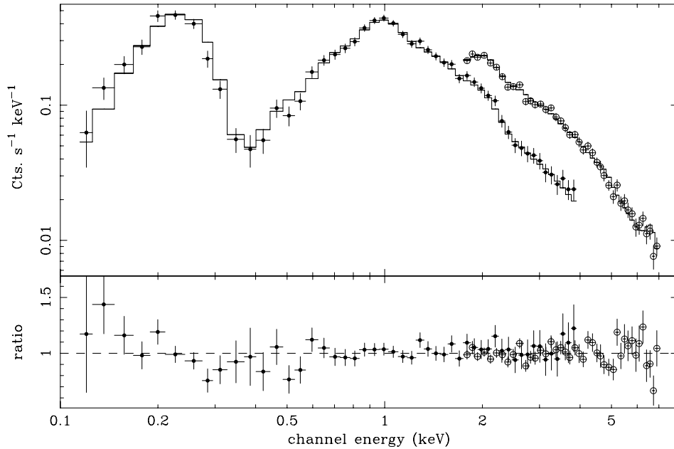
Fig. 3. LECS+MECS spectra for the whole data set with N_{\text{H}} free to vary. The ratio between the data and the MEKAL two-temperature best-fit model are shown in the lower panel.
