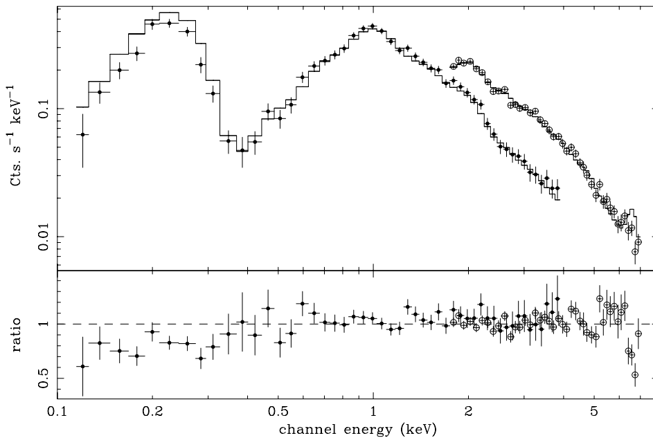
Fig. 2. LECS+MECS spectra for the whole data set with N_{\text{H}} frozen to 5 \times 10^{18} cm ^{-2} . The ratio between the data and the MEKAL two-temperature best-fit model are shown in the lower panel.
