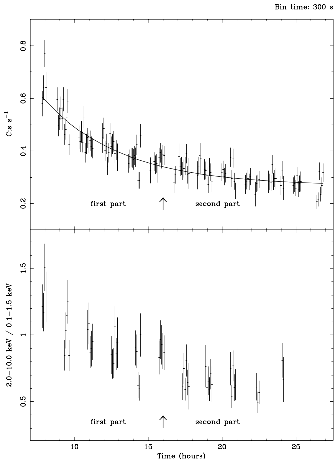
Fig. 1. Top panel: II Peg MECS light curve in the energy range from 2 to 10 keV. The solid line shows the best fit exponential plus constant curve. The quiescent flux at the end of the observation turns out to be \sim 0.27 Cts s^{-1} and the decay time \sim 5.3 hours. The background has been stable during the observation and amounts to roughly one hundredth of the source flux in the MECS cameras. Bottom panel: Hardness ratio between 2.0–10.0 keV (MECS) data and 0.1–1.5 keV (LECS) data. The binning time is 300 s. The observation started on December 5 1997 and the arrow signs the separation between the first and the second part of the observation considered in the spectral analysis.
