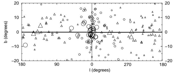
Fig. 4. Angular distribution in galactic coordinates for globular clusters (circles) and old open clusters (triangles) within |b| < 20^\circ . The symbol size is proportional to reddening derived from the stellar content: (i) large corresponds to E(B-V) > 1.0 ; (ii) intermediate 0.2 \leq E(B-V) \leq 1.0 ; and (iii) small E(B-V) < 0.2 .
