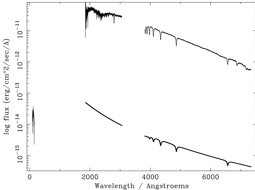
Fig. 5. Left to right: EUV, UV and optical spectra of 16 Dra, shown together with a white dwarf model for T_{\text{eff}} = 31,900\text{K} and \log g = 8.5 . The B9.5V star clearly dominates the UV and optical flux, and the white dwarf is only detectable in the EUV. The UV spectrum was extracted from the IUE final archive (LWP18244). The optical spectrum was obtained on 1997 March 17 at the Russain Academy of Sciences' Special Astrophysical Observatory's 6m telescope, located in the Karachaevo-Cherkesia region of southern Russia.
