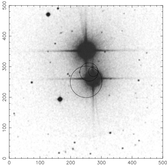
Fig. 1. Optical image of the 16 Dra system from the Digitized Sky Survey. The field is 8 \times 8 arcmin. The lower of the bright stars is 16 Dra. The upper bright star is the 17 Dra A/B pair, unresolved here but in fact separated by 3.2 arcsec. The circles denote, in decreasing order of size, the ROSAT WFC, EUVE and ROSAT PSPC source error boxes.
