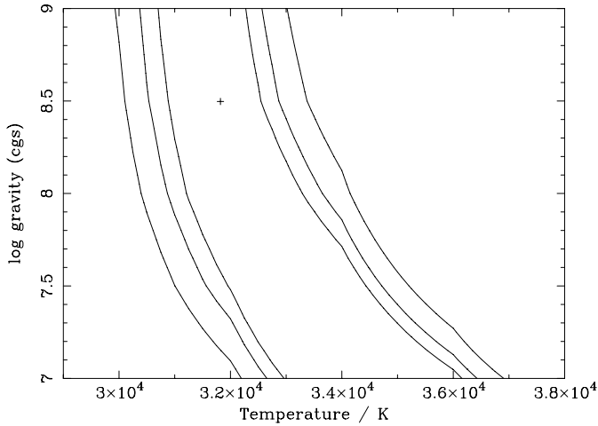
Fig. 3. Confidence contours for the spectral fit to the EUVE data, at 66%, 90% and 99% in the (T_{\text{eff}}, \log g) plane.
