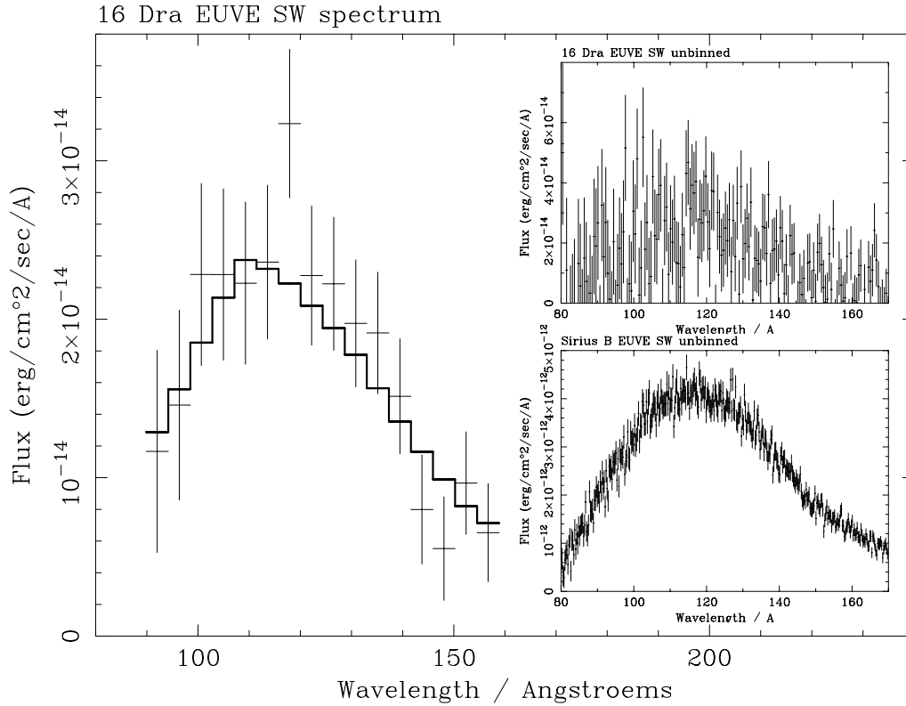
Fig. 2. EUVE short wavelength spectrum of 16 Dra, shown together with a pure-H white dwarf + ISM model (solid line) for \log g = 8.5 , T_{\text{eff}} = 31,900\text{K} , N_{\text{HI}} = 8.2 \times 10^{18} \text{ atoms cm}^{-2} , N_{\text{HeI}} = 9 \times 10^{17} \text{ atoms cm}^{-2} , and N_{\text{HeII}} = 3 \times 10^{17} \text{ atoms cm}^{-2} . Inset (upper): the same data, displayed at the instrument resolution of \approx 0.5\text{\AA} . Inset (lower): EUVE short wavelength spectrum of Sirius B, for comparison.
