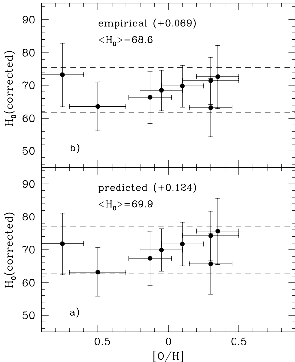
Fig. 6. a As in Fig. 5b, but with the predicted metallicity correction \Delta h_0/\Delta[\text{O}/\text{H}] \sim +0.124 \text{ dex}^{-1} ; b As below, but with the metallicity correction \Delta h_0/\Delta[\text{O}/\text{H}] \sim +0.069 \text{ dex}^{-1} , as suggested by the dotted line in Fig. 5a.
