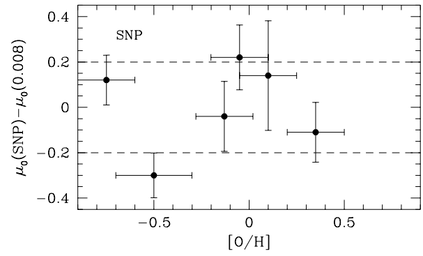
Fig. 2. As in Fig. 1, but with the Cepheid distances by the SNP group.
