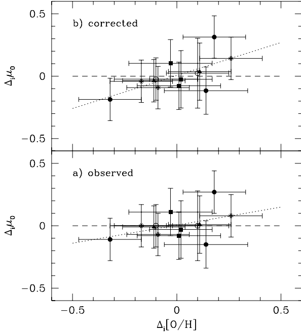
Fig. 4a and b. a Residuals of each galaxy from the average true distance modulus and O/H metallicity of the host cluster or group. Symbols as follows: Fornax cluster: filled circles, NGC 3184 group: triangles, Leo I group: squares, M87 sub-cluster: open circles, NGC 4472 sub-cluster: asterisks. The dotted line is the best fit to the points [Eq. (4)]. b As below, but with the Kennicutt et al. (1998) metallicity correction to the absolute distance moduli [Eq. (5)].
