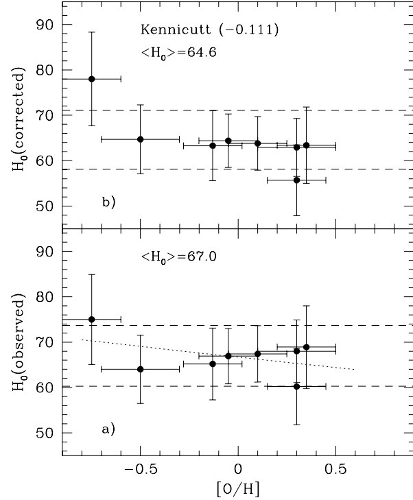
Fig. 5. a The KP H_0(V) values from LMC-based Cepheid distance to the eight SNIa calibrating galaxies. The average value is labelled. The dashed lines depict the uncertainty of 10%. The dotted line depicts Eq. (6) in the text; b As below, but with the Kennicutt et al. (1998) metallicity correction to the absolute distance moduli. The resulting correction to H_0 is \Delta h_0/\Delta[O/H] \sim -0.111 \text{ dex}^{-1} (see text).
