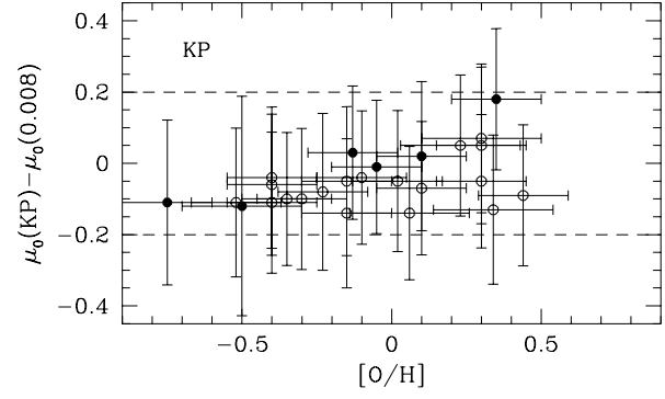
Fig. 1. The difference between the empirical Cepheid distance by KP studies and the predicted value with Z = 0.008 , plotted against the O/H metallicity of the host galaxy. The Cepheid samples are original KP data (open circles) or refer to SNP galaxies extracted from the HST archive and re-processed by the KP team (filled circles). The two dashed lines depict a discrepancy on the distance of the order of \pm 10\% .
