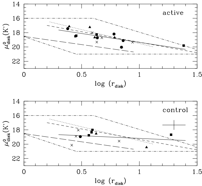
Fig. 2. Same as Fig. 1 but for the disk component.
