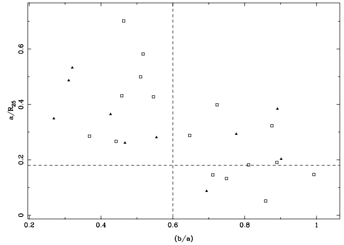
Fig. 5. Relation between primary bar strength and length for active (squares) and control (triangles) galaxies. The limits for strong and long bars as defined by Martinet & Friedli (1997) (see text) are given as dashed lines.
