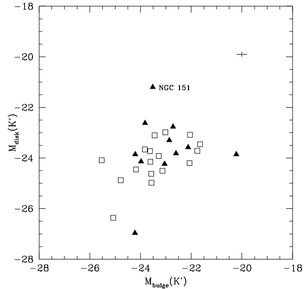
Fig. 3. Relation between bulge and disk absolute magnitudes in K'. Active and non active galaxies are indicated with empty squares and full triangles respectively. Typical errors are represented by the cross.
