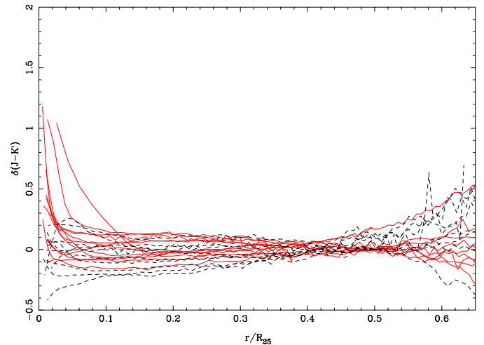
Fig. 8. Normalized color gradients (\delta(J-K')(u) = (J-K')(u) - (J-K')(0.5)) , with u=r/R_{25} for active (full line) and control (dashed line) galaxies.
