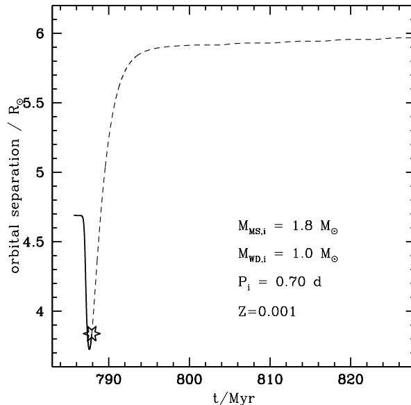
Fig. 6. Evolution of the orbital separation as function of time for System No. 61.
