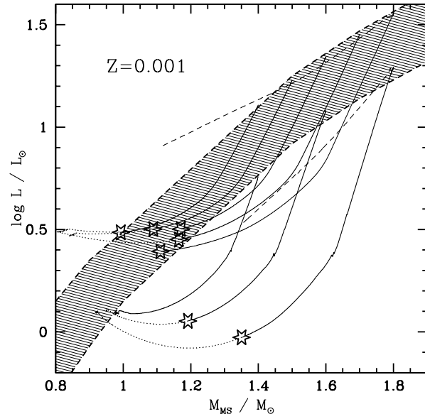
Fig. 19. Same as Fig. 18, but for our Z = 0.001 Z_{\odot} Systems No. 60, 61, 63, 64, 65, 67, 68, and 70. The evolution of the nuclear luminosity is shown for Systems No. 60 (lower line) and No. 61 (upper line).
