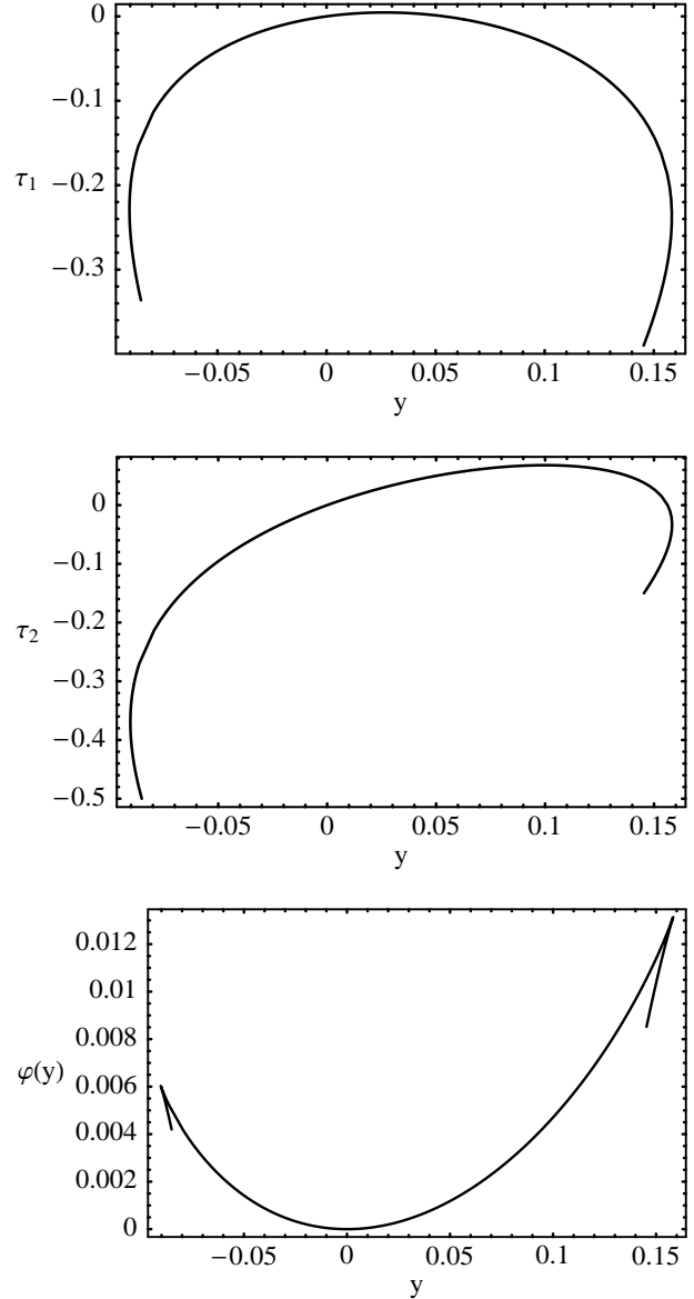
Fig. 2. Shape of the functions \tau_1(y) and \tau_2(y) for the two-cell compensated window function ( y \equiv -\lambda\sigma^2 ). The computations have been done for a power law spectrum for n = -1.5 . The solution for \tau has been extended beyond the singularity to show explicitly that the singularities are due to double solution in y .
