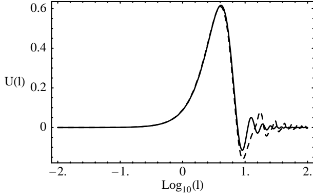
Fig. 1. Shape of the filter functions we use in Fourier space. The solid line corresponds to the shape proposed by Schneider, Eq. (12), multiplied by 1.459 and the dashed line corresponds to the compensated filter we introduce in this paper, Eq. (15).
