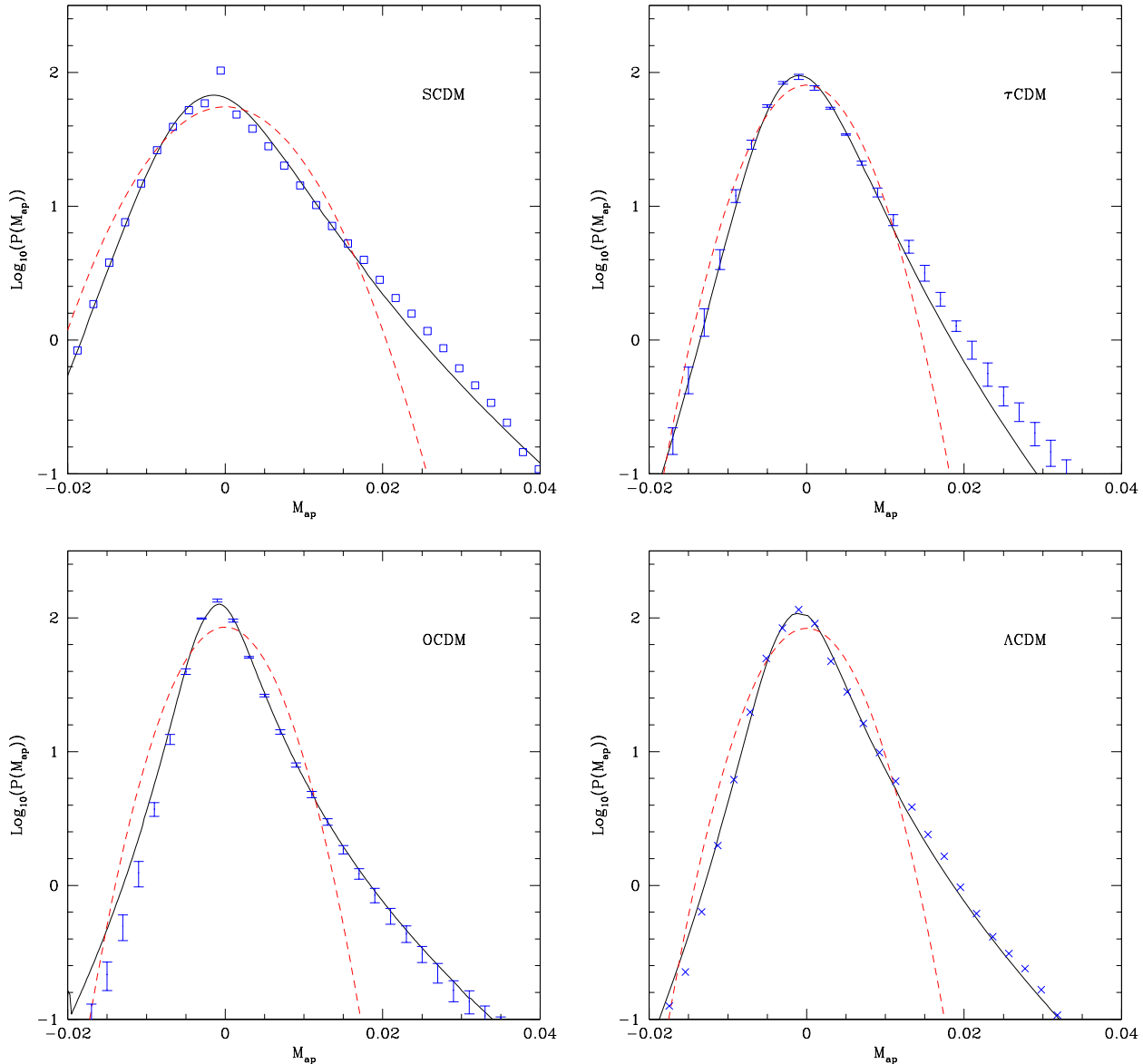
Fig. 8. The aperture mass PDF for a source at redshift z_s = 1 for 4 cosmologies and with the angular window \theta = 4' . The dashed line shows the Gaussian which has the same variance. The points show the results of N-body simulations from Jain et al. (2000). Results for \Lambda CDM and \tau CDM models have been directly taken from Reblinsky et al. (1999).
