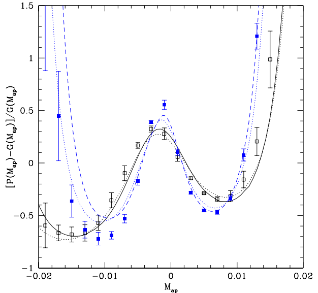
Fig. 9. The relative difference [P(M_{\text{ap}}) - G(M_{\text{ap}})]/G(M_{\text{ap}}) of the aperture mass PDF P(M_{\text{ap}}) with respect to the Gaussian G(M_{\text{ap}}) . The variance of the Gaussian is taken from the simulations. As in Fig. 8 we consider a source at redshift z_s = 1 with the angular window \theta = 4' . We display our results for the \tau CDM (solid line) and OCDM (dashed line) cosmologies. The dotted lines correspond to the same cosmologies with \kappa = 0.88 (see main text). The points show the results of N-body simulations from Jain et al. (2000).
