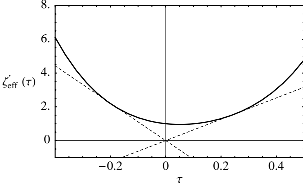
Fig. 3. Geometrical representation of Eq. (86). The function \tau(y) is given by the intersection of the line -\tau/y with the curve \zeta'_{\text{eff.}}(\tau) . Singularities appear when both curves are tangential, as shown in the figure.
