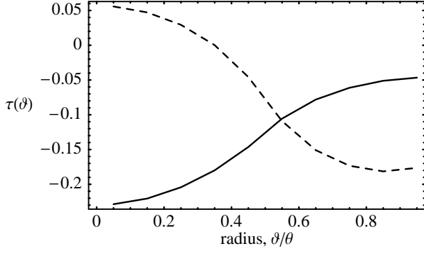
Fig. 4. Profile of the \tau function as a function of the angular radius. The two plots correspond to the two singularities, y_{s-} for the solid line and y_{s+} for the dashed line.
