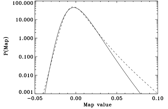
Fig. 7. Same as previously with the nonlinear model but with cell radius ratio of 10 instead of 2.
