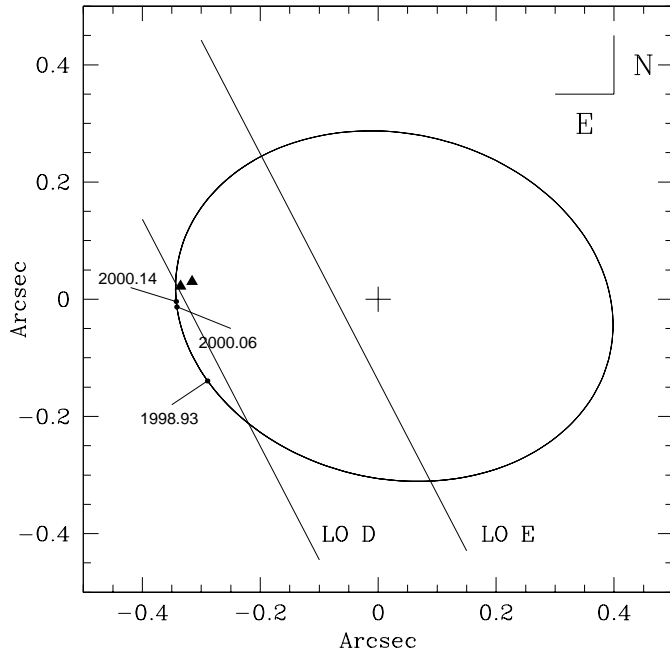
Fig. 4. The orbit of \zeta Cnc D around the C component, computed from the orbital parameters and the mass ratio given by H96 (solid line). The D positions observed by HGM are superimposed as solid triangles, together with the lines of possible solutions for the positions of the D and E components from Table 2. Also marked are the epochs of the AO and LO observations on the H96 orbit (dots labeled by dates).
