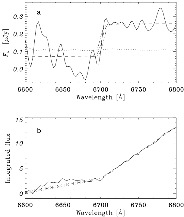
Fig. 7a and b. a A region of the spectrum, centered on the Ly \alpha absorption edge and smoothed to a resolution of 13 Å. The dotted line gives the noise per bin, while the dashed curve is a model absorption edge spectrum corresponding to a redshift of 4.511, and redshifts of 4.509 and 4.513 (dot-dashed curves). b The integrated flux of the full resolution spectrum and the model absorption edge spectra shown in a . The integrated flux is normalized to a common level at 6750 Å.
