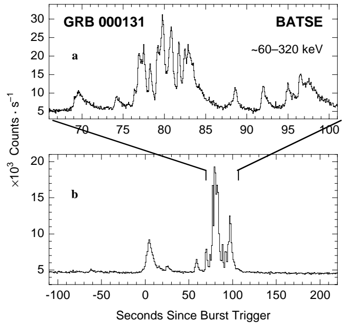
Fig. 1a and b. Gamma-ray light curve of GRB 000131 recorded by the BATSE Large Area Detectors (LADs). b shows continuously recorded data with 1024 ms time resolution, a shows an enlargement of the most intense interval using triggered data with 64 ms time resolution. In both cases, data from the two most brightly illuminated LADs have been summed. Energy channels for the different data types and detectors have been chosen to approximately match (within a few percent) the energy range 60–320 keV.
