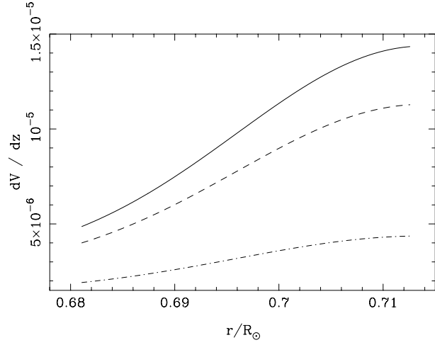
Fig. 1. The shear rate dV/dz with respect to radius beneath the convection zone for the colatitudes \theta = 90^\circ (full), \theta = 60^\circ (dashed) and \theta = 30^\circ (dash-dot-dash).
