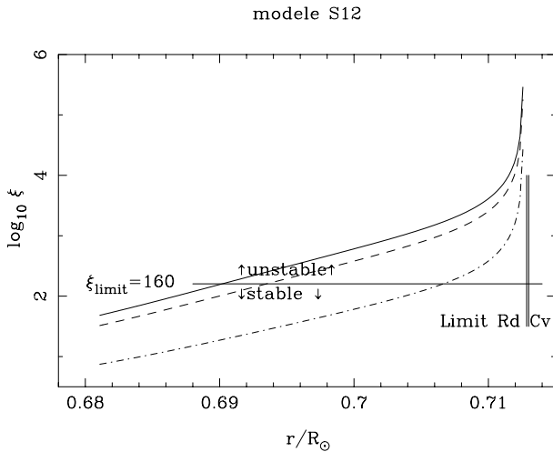
Fig. 2. For the colatitudes \theta = 90^\circ (full), \theta = 60^\circ (dashed) and \theta = 30^\circ (dash-dot-dash), stable and unstable regions beneath the tachocline located about at the limit Rd Cv between the convection zone and the radiative interior.
