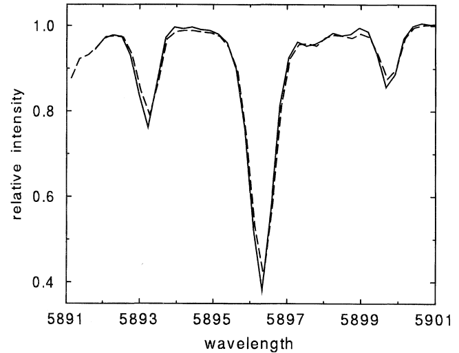
Fig. 4. A part of the spectrum of the zero-field standard o UMa solid line – right circular polarization, dashed line – left circular polarization
