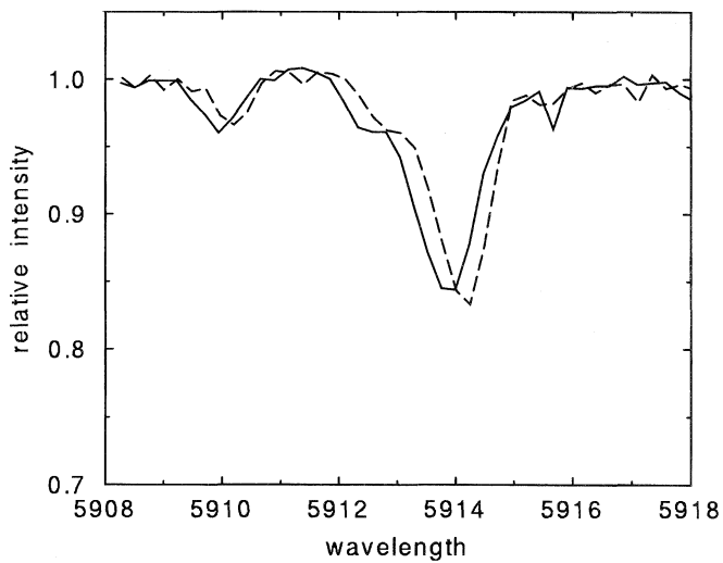
Fig. 3. A part of the spectrum of the magnetic star 53 Cam. solid line – right circular polarization, dashed line – left circular polarization
