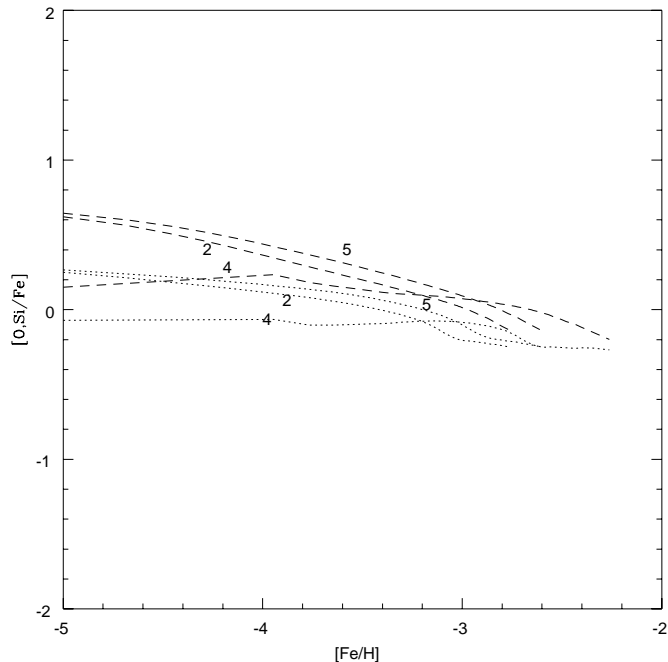
Fig. 2. Predicted and observed [O,Si/Fe] versus [Fe/H] . The long-dashed lines refers to O, whereas the short-dashed lines refers to Si. The model numbers are indicated on each curve.
