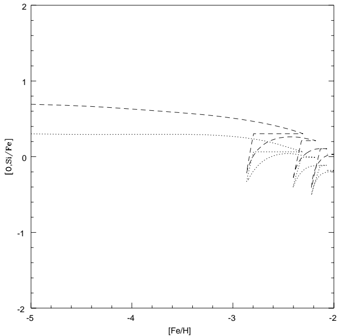
Fig. 4. The same as Fig. 2 but for model 6. The dashed lines refer to O, whereas the dotted lines refer to Si.
