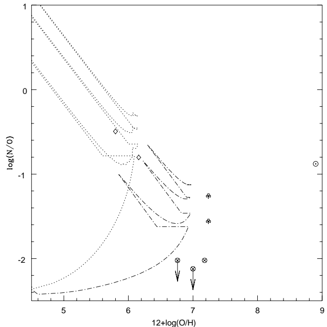
Fig. 3. The same as Fig. 1 but here are shown only the predictions of models 6 (dashed-dotted line) and 7 (dotted line).
