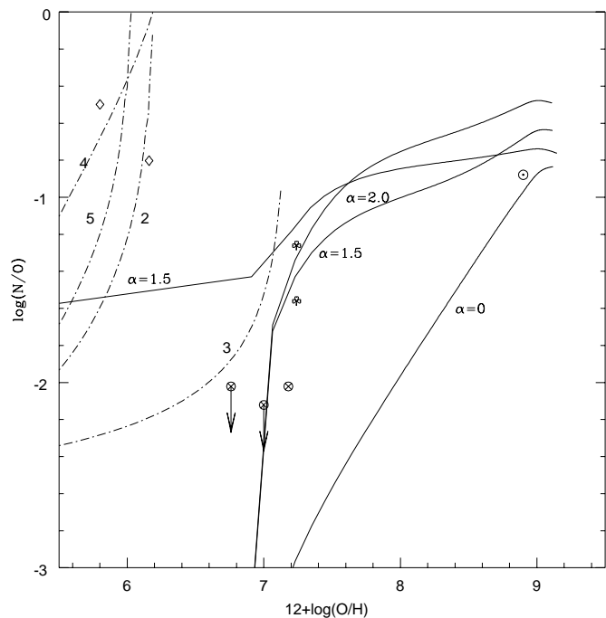
Fig. 1. \log(\text{N}/\text{O}) vs. 12+\log(\text{O}/\text{H}) as predicted by different models of chemical evolution. In particular, the continuous lines refer to a model for the solar neighbourhood, as described in the text, for different prescriptions concerning the nucleosynthesis of N. The value of the \alpha parameter in Renzini and Voli (1981) is indicated on each curve; \alpha=0 means only secondary N in low and intermediate mass stars, \alpha=1.5 and 2.0 indicate different amounts of primary N produced during the third dredge-up according to the efficiency of convection. The line with a plateau and labelled \alpha=1.5 represents a model where N is assumed to be primary in massive stars (in all the other models is secondary) plus primary N from intermediate mass stars with \alpha=1.5 . The dash-dotted lines are the predictions of starburst models with only one burst, as described in Table 3. The symbols refer to measurements of N/O and O/H ratios in the sun and in the DLA shown in Table 4. In particular, the romb with the highest N/O is the system observed by Molaro et al. (1996) whereas the other romb is the DLA system observed by Green et al. (1995). The clovers refer to different measurements for IZw18, the one with the highest N/O is from Skillman and Kennicutt (1993), whereas the other is from Dufour et al. (1988). The crossed circles are the DLA systems discussed in Pettini et al. (1995) and Lipman (1995).
