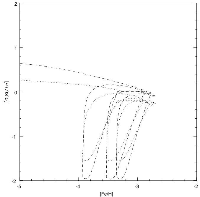
Fig. 5. The same as Fig. 2 but for model 7. The dashed lines refer to O, whereas the dotted lines refer to Si.
