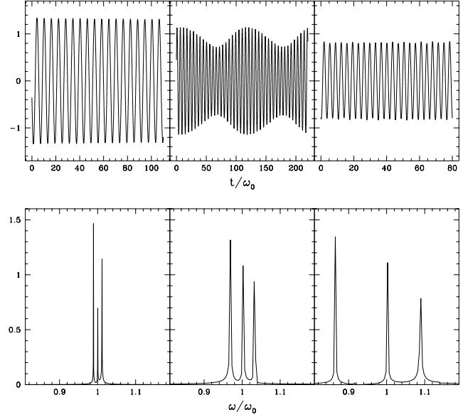
Fig. 4. top from left to right: Temporal behavior of the component z(t) (Eq.21c) for \delta\omega/\kappa_0 = 0.5, 4, 50 with \kappa_0/\omega_0 = 10^{-2} . bottom: Corresponding Fourier amplitude spectra, see text.
