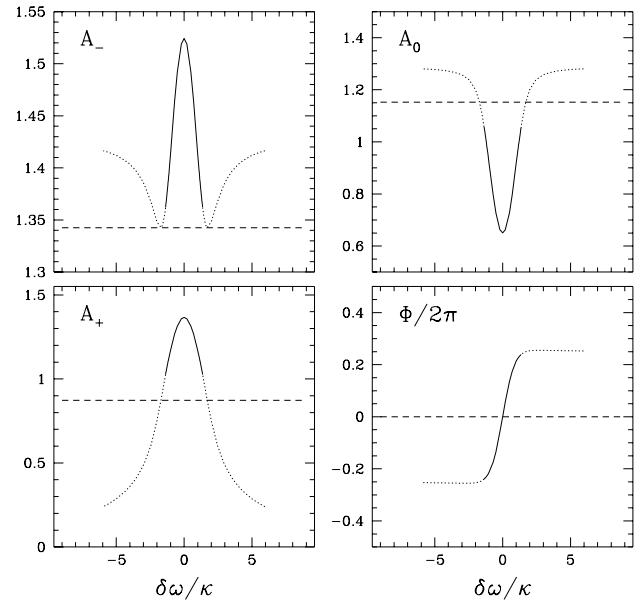
Fig. 3. Amplitudes and phase \Phi of a resonant triplet \ell = 1 as the resonance detuning parameter \delta\omega/\kappa_0 is increased; solid line : stable, dashed : unstable solution; Dotted lines : amplitudes of the NR triplet FP.
