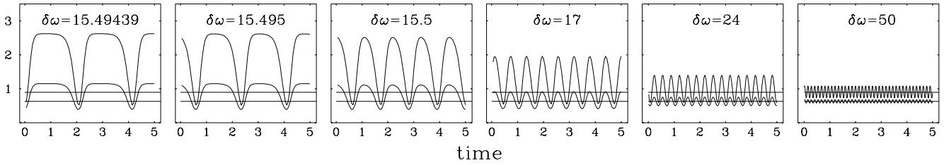
Fig. 2. 2:1 Resonance: Amplitude modulations, as a function of the resonance detuning parameter \delta\omega in units of \kappa_0 ; the large and small amplitudes correspond to modes a and b , resp.
