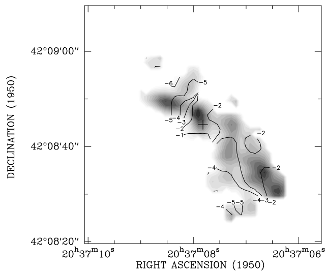
Fig. 6. Map of the 2_0 \rightarrow 1_0A^+ methanol transition emission in DR 21-W. The grey-scale map shows the peak intensity (from gaussian fits) in steps of 0.025 Jy starting at 0.05 Jy. The contours show the center velocity in steps of 1 kms -1 , from -6 to -1 kms -1 . The maser position is shown by a cross.
