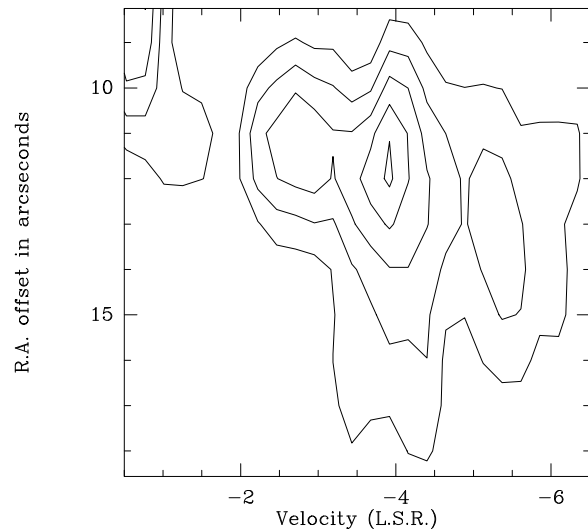
Fig. 4. Velocity-position plot of the 2_0 \rightarrow 1_0 A^+ methanol transition in MM1. The cut is along the right ascension axis and the emission was summed over declinations 42^\circ 12' 09.6'' to 42^\circ 12' 12.6'' . The ordinate axis is in right ascension arcseconds offset from the field center.
