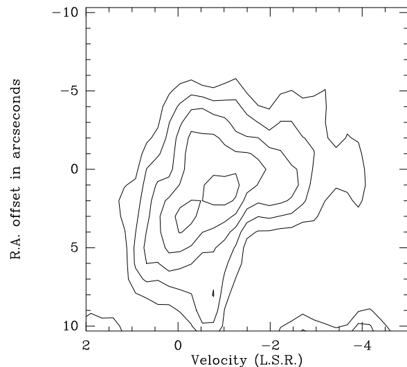
Fig. 5. Velocity-position plot of the 2_0 \rightarrow 1_0 A^+ methanol transition around DR 21(OH)-2. The cut is along the right ascension axis and the emission was summed over declinations 42^\circ 12' 07.6'' to 42^\circ 12' 12.6'' . The ordinate axis is in right ascension arcseconds offset from the field center.
