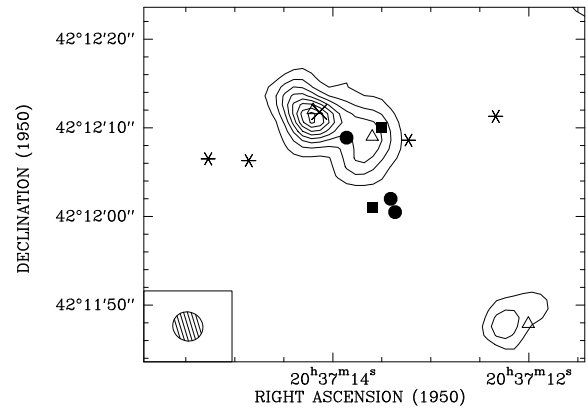
Fig. 1. CLEANed map of the 3.1mm continuum emission towards DR 21(OH). Contours are drawn in steps of 10 mJy/beam starting at 10 mJy/beam. We have corrected for primary beam attenuation. The 3.5'' \times 3.2'' beam is drawn in the bottom left corner. Indicated are the positions of the 8_0 \rightarrow 7_1 A^+ methanol masers (Stars; PM90), the H 2 O maser groups (Filled circles; Mangum et al. 1992), the OH maser (Cross; Norris et al. 1982), the H 2 CO emission peaks (Filled square; Johnston et al. 1984) and the 2.7mm continuum emission peaks (Unfilled triangles; Mangum et al. 1991).
