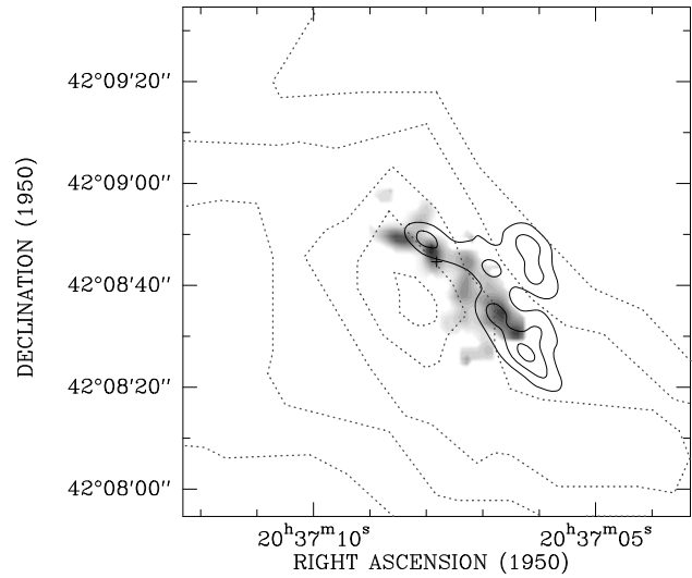
Fig. 8. Methanol, CS and vibrationally excited \text{H}_2 emission in DR 21-W. The methanol emission is shown by the same grey-scale map as in Fig. 6. Solid contours represent CS(2-1) emission (PM90) and dashed contours represent the 2.2 \mu\text{m} emission from shock-excited \text{H}_2 (Garden et al. 1986).
