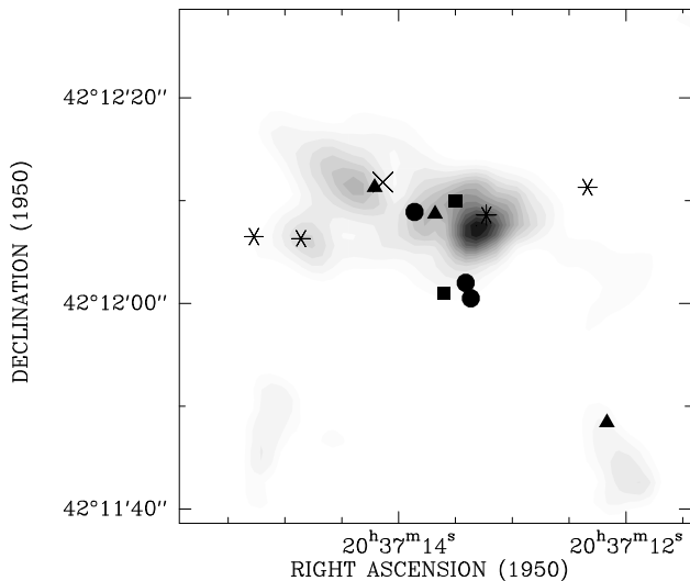
Fig. 3. Map of the 2_0 \rightarrow 1_0 A^+ methanol transition emission in DR 21(OH). The grey-scale map shows the integrated intensity of this transition in steps of 0.3 \text{ Jy km s}^{-1} starting at 0.5 \text{ Jy km s}^{-1} . The symbols are the same as the ones used in Fig. 1, except that the continuum emission peaks are the ones derived from the observations reported in this paper (Table 1), and are indicated by filled triangles.
