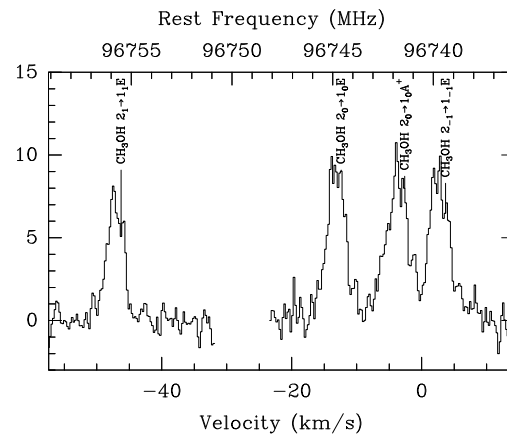
Fig. 7. Spectrum of the four methanol transitions towards MM1. The spectrum is an average over a box of 1'' around the continuum position from Table 1. The ordinate is brightness temperature (1 K = 91 mJy/beam).
