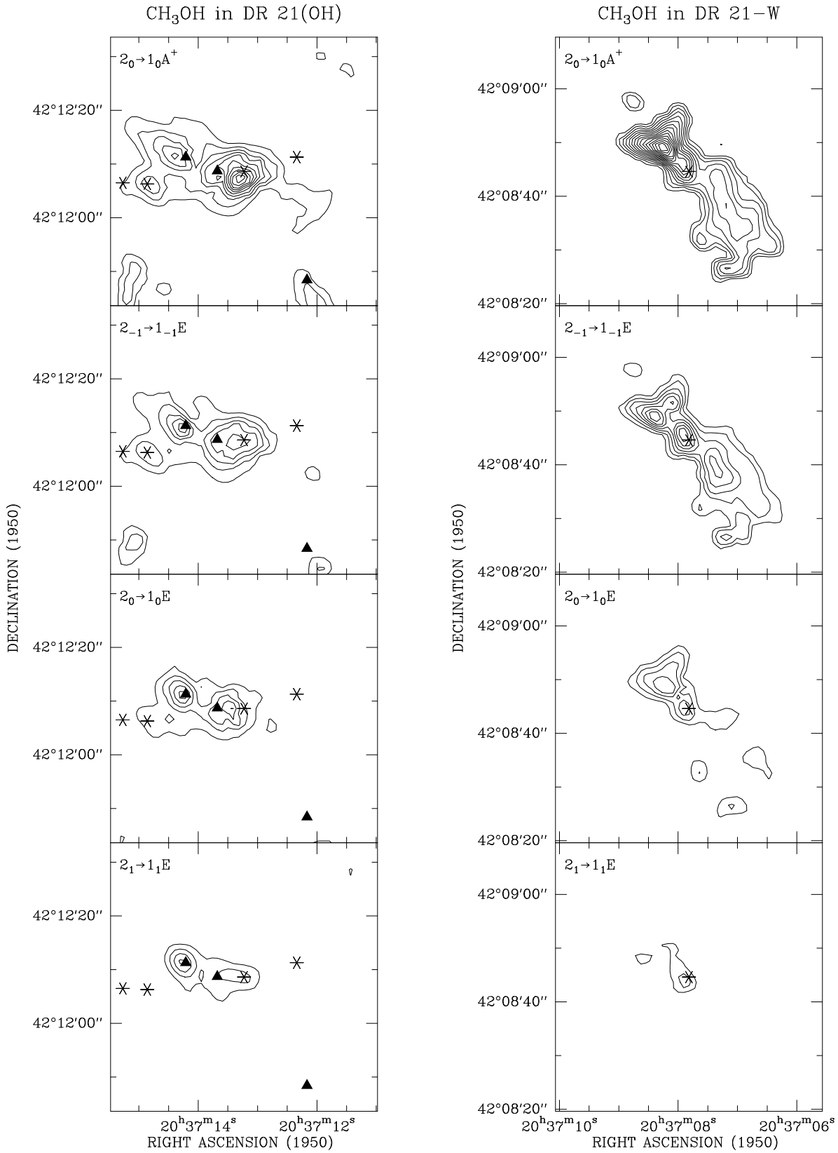
Fig. 2. Contour maps of the methanol integrated intensity (resulting from gaussian fits) in each transition. The levels are from 0.5 to 6 \text{Jy.kms}^{-1} in steps of 0.5 \text{Jy.kms}^{-1} for DR 21(OH), and from 0.1 to 1.7 \text{Jy.kms}^{-1} in steps of 0.1 \text{Jy.kms}^{-1} in DR 21-W. The stars mark positions of 8_0 \rightarrow 7_1 A^+ methanol masers from PM90, and the filled triangles, the positions of the continuum emission peaks derived from our observations (Table 1).
