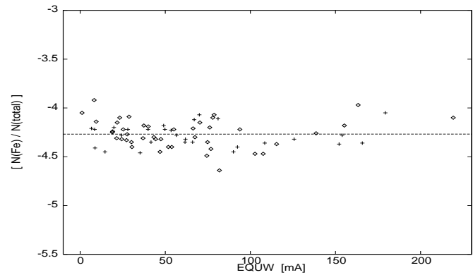
Fig. 6. Confirmation of the microturbulent velocity. Abundances versus equivalent width of 41 Fe I (diamonds) and 28 Fe II lines (crosses) are plotted for v_{\text{micro}} = 0.0 km s -1 .
