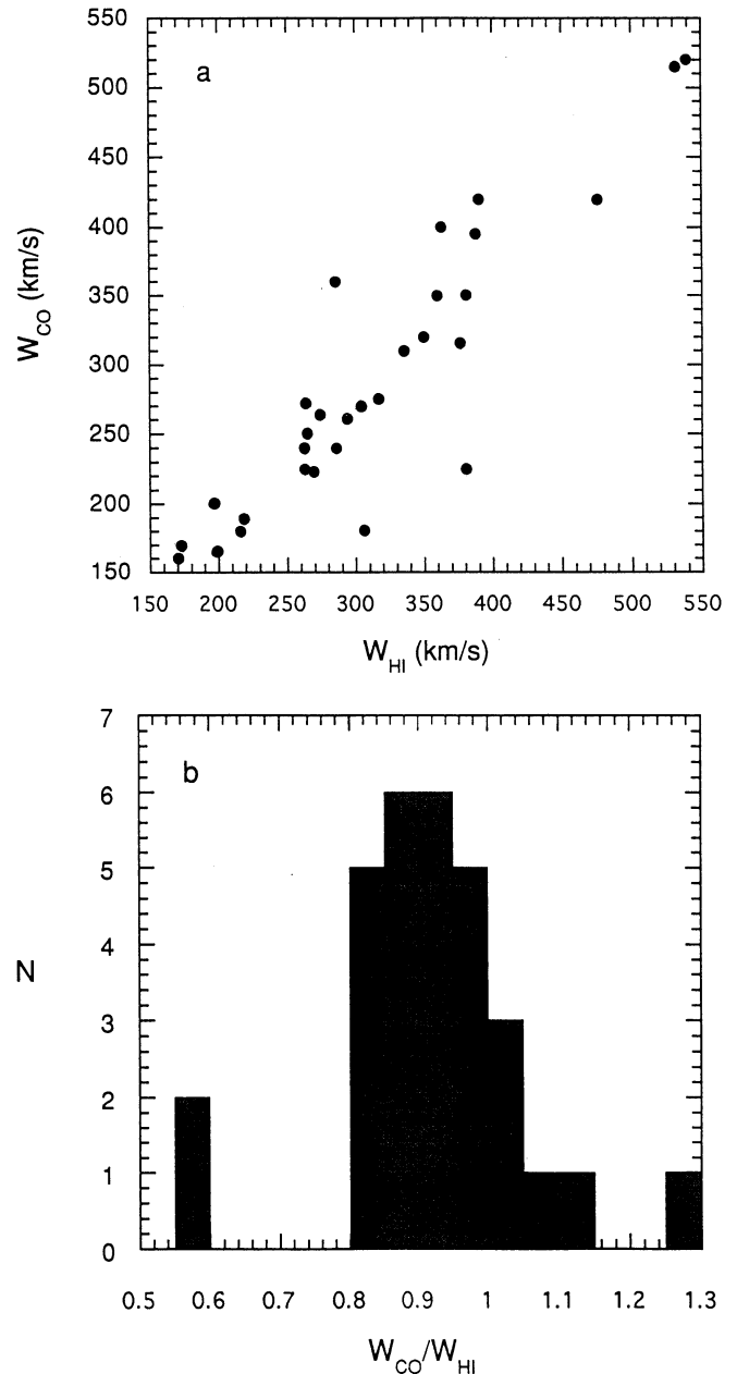
Fig. 1. a CO vs HI linewidths and b a histogram of galaxy numbers vs W_{CO}/W_{HI}
