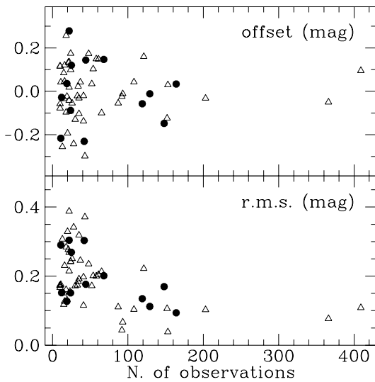
Fig. 2. Offset and rms. from the mean visual lightcurve of YY Her in quiescence for the AAVSO (open triangles) and AFOEV (filled circles) observers with more than 10 recorded observations.
