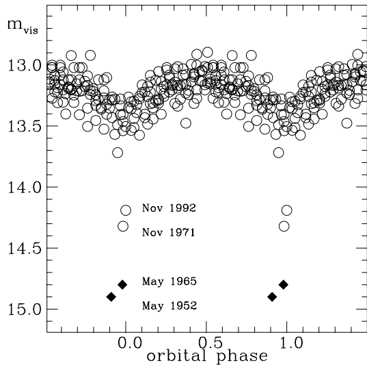
Fig. 5. Phase plot of the quiescence visual lightcurve of YY Her according to ephemeris (2). The solid diamonds are the two minima in the m_{pg} lightcurve of Fig. 3 at JD=2434141 and 2438902 are plotted for reference purposes.
