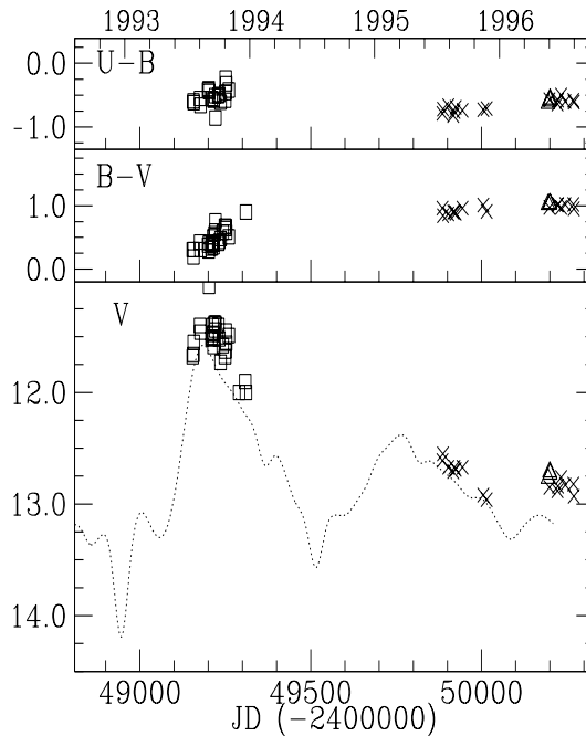
Fig. 4. UBV photoelectric photometry during the 1993-95 outburst. The dotted line is plotted for reference purposes and shows a spline fit to the binned AAVSO+AFOEV lightcurve. Open squares : AFAM; Crosses : Crimean Astronomical Observatory
