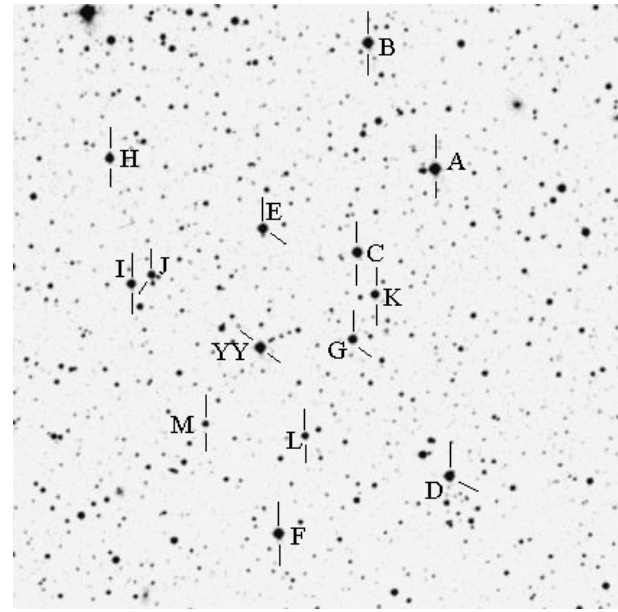
Fig. 1. Identification of the comparison stars in Table 1 (chart from the digitized version of the Palomar Observatory Sky Survey; field 12 arc min).
