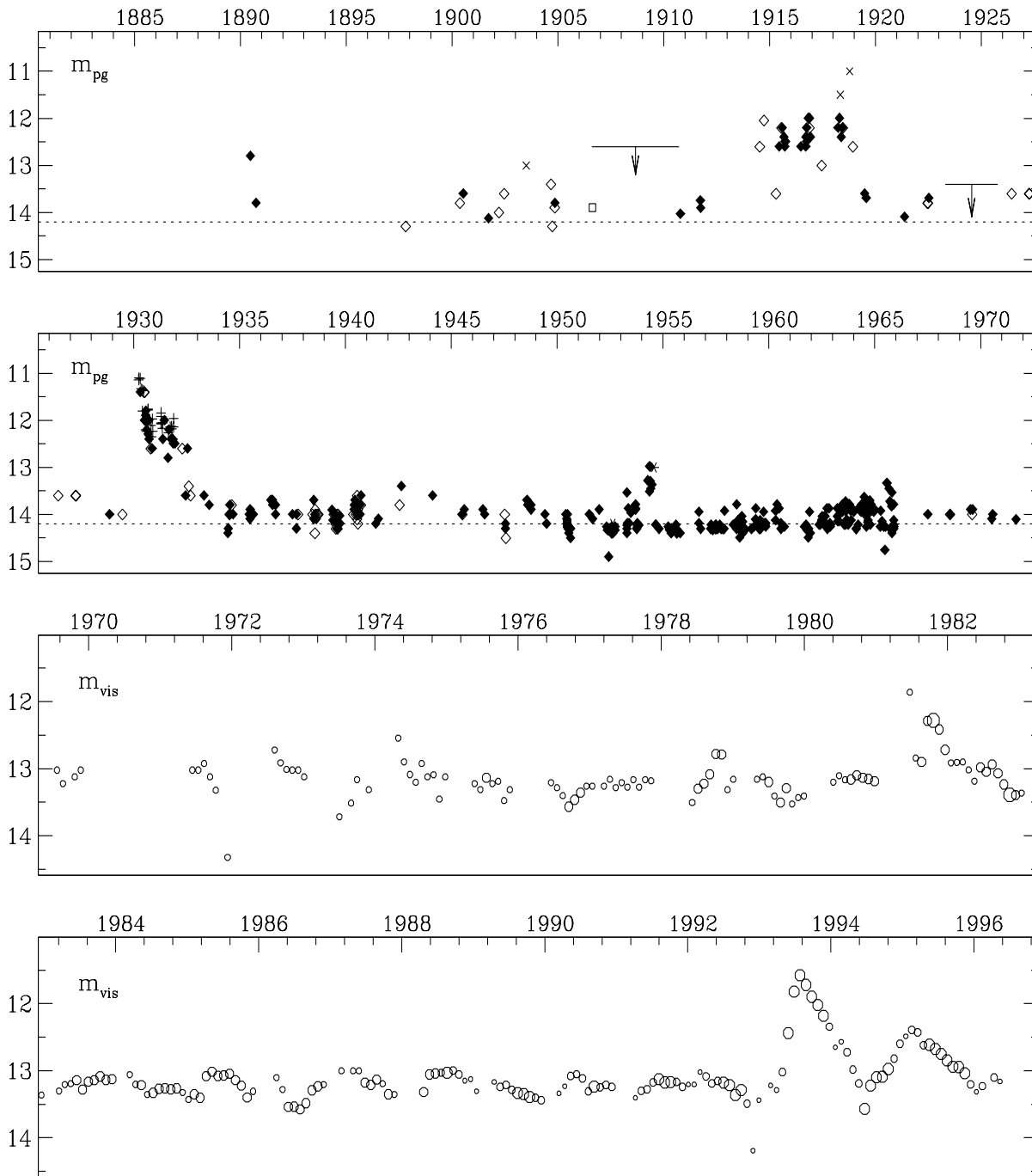
Fig. 3. The 1890-1996 lightcurve of YY Her. m_{pg} Panels. The dotted line is the quiescence B magnitude from photoelectric photometry in Table 2. Upper limits from Table 6 are omitted for plot clarity. Filled rhombs : our data from Table 6; Open rhombs : uncertain values from Table 6; Crosses : from Wolf (1919); Plus signs : from Plaut (1932); Asterisks : estimates on the POSS blue prints; Filled squares : from Herbig (1950); Open square : estimate on the Carte du Ciel. m_{vis} Panels. The circle dimension is proportional to the number N of individual estimates in the given 30-day bin. Smallest circles refer to N \leq 5 , intermediate to 5 < N < 30 , and the largest one to N \geq 30 .
