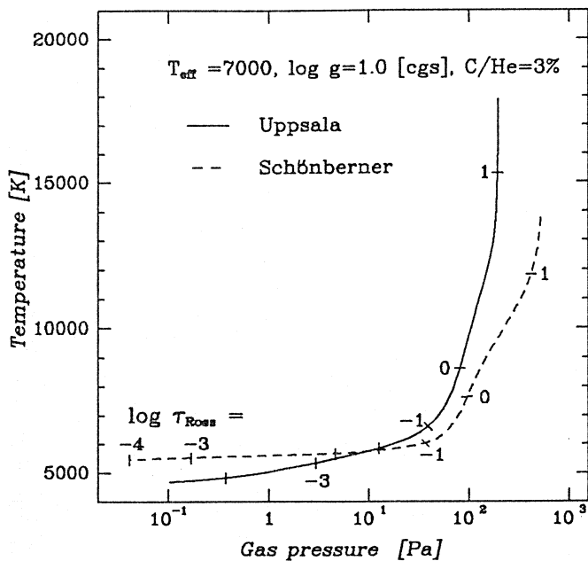
Fig. 6. Comparison of a line-blanketed model atmosphere (solid) with a Schönberger model (dashed) with the same parameters ( T_{\text{eff}} = 7000 , \log g = 1.0 [cgs] and C/He = 3%). Rosseland optical depths are marked along the curves
