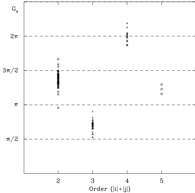
Fig. 1. A well defined separation is obtained when plotting the generalized phase values G_{i,j} as function of order
