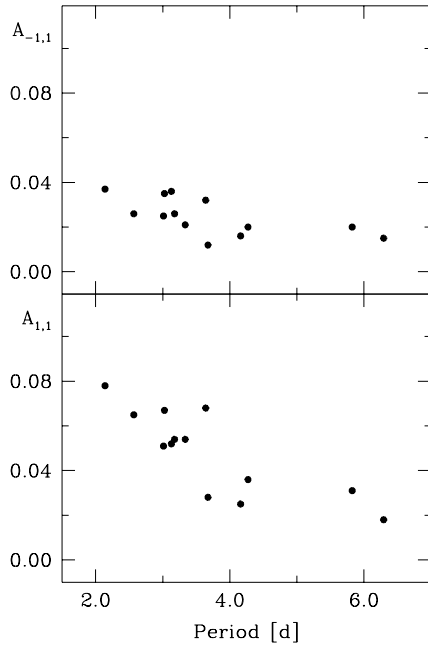
Fig. 3. The amplitude of the cross-coupling terms f_1 + f_2 decreases towards longer periods and it reaches its minimum at P \sim 6.0 d (lower panel); the amplitude of the f_2 - f_1 term is small over the whole range of period values
