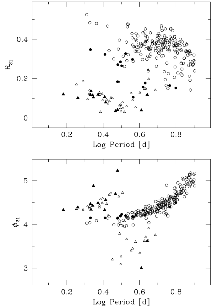
Fig. 4. The Fourier parameters \phi_{21} and R_{21} provide a powerful discrimination between F and 1O pulsators when plotted versus Period. Dots: single-mode Classical Cepheids. Triangles: s -Cepheids. Filled dots: Fundamental radial mode of DMCs. Filled triangles: 1O radial mode of DMCs
