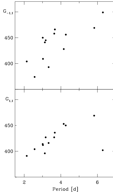
Fig. 2. Generalized phase differences of the most important cross-coupling terms ( f_1 + f_2 and f_2 - f_1 ) of DMC light curves shown as function of pulsation period. While the G_{-1,1} progression does not show any particularity, the G_{1,1} progression seems to be interrupted at P \simeq 6.0 d, as indicated by the last point (V367 Sct)
