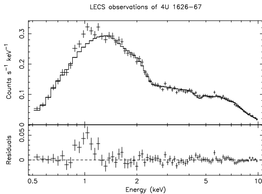
Fig. 1. Phase averaged data and folded model for 4U 1626–67. The data are described by a model consisting of a blackbody of kT = 0.33 keV, a power-law of \alpha = 0.61 , an emission-line centered on 1.05 keV and low energy absorption. For illustrative purposes, the line intensity is set to zero. The lower panel shows the residuals
