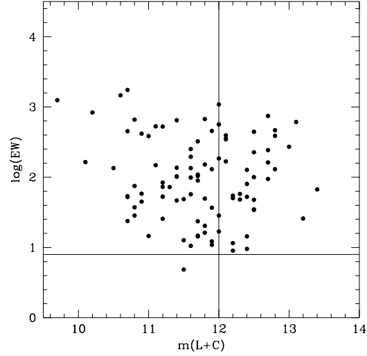
Fig. 1. A plot of \log(\text{EW}) versus m_{L+C} , where EW are the equivalent widths in \text{\AA} and m_{L+C} is the flux in the emission-line plus the flux in the continuum under the line, transformed in a magnitude scale (see (1)). With the vertical line we delimit the complete sample from the incomplete one and with the horizontal line we trace the threshold below which the ELGs are no more seen by our survey.
