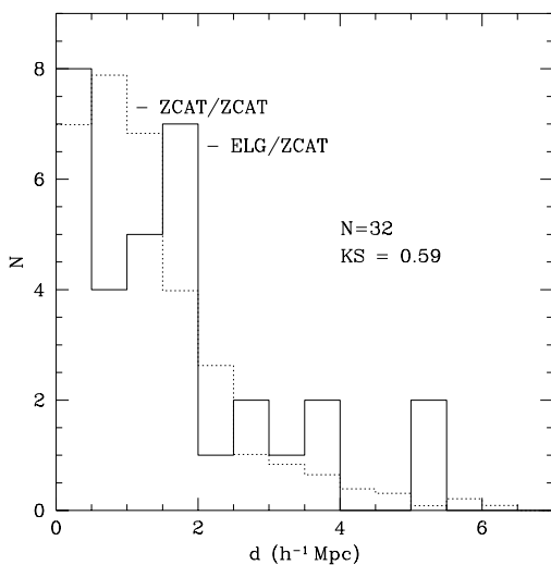
Fig. 5. The nearest neighbour distributions. The ELG/ZCAT separations are plotted with solid line and the comparison ZCAT/ZCAT distribution with dashed lines.
