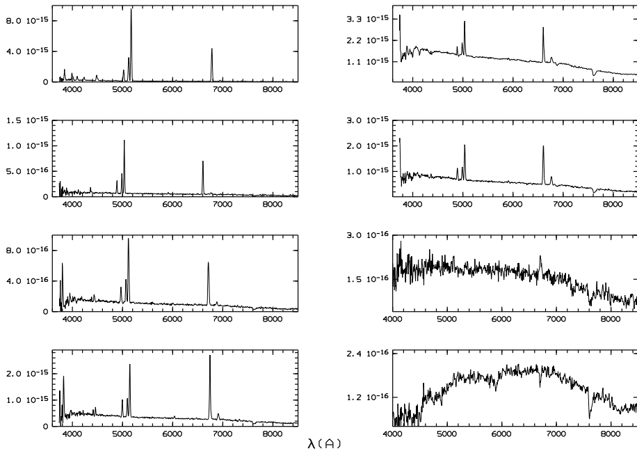
Fig. 6. Spectra of void galaxies. The y-axes contain the fluxes per unit of wavelength, F_{\lambda} ( \text{erg sec}^{-1} \text{cm}^{-2} \text{\AA}^{-1} ) while the x-axes contain the wavelength, \lambda ( \text{\AA} ).
