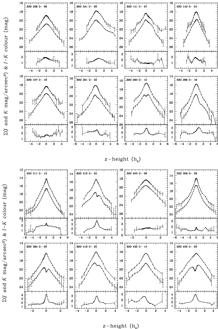
Fig. 10. Central I and K -band vertical profiles for the total sample, and their corresponding I-K colours
