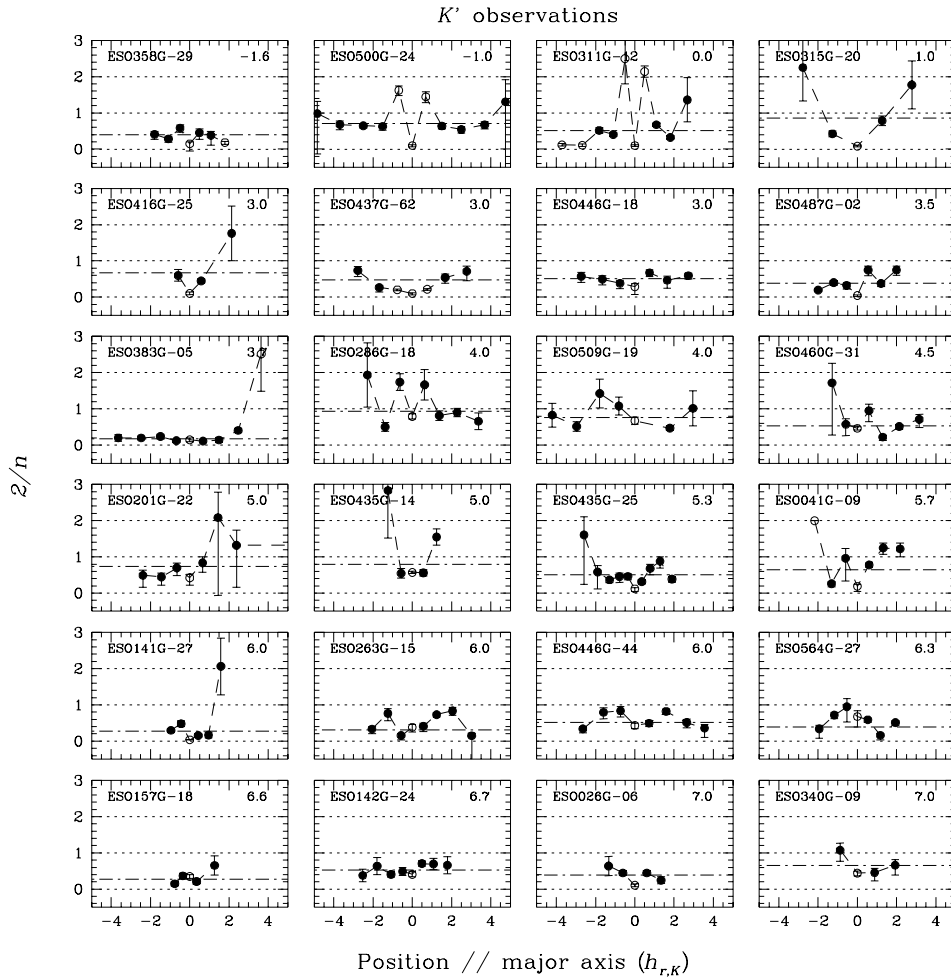
Fig. 6. Best-fitting exponents determining the sharpness of the peak in the galaxies’ vertical luminosity profiles. The galaxies are ordered by revised Hubble type, which is shown in the upper right corner of each panel. The dotted lines indicate the levels corresponding to an exponential profile ( 2/n = 0 ), an isothermal profile ( 2/n = 2 ), and the intermediate sech( z ) distribution ( 2/n = 1 ). The dash-dotted line represents the mean best-fitting value for the galaxies’ disks, obtained by averaging the filled data points; the open circles were not taken into account when determining these levels, because of either bulge light contamination or an excessively high \chi^2 value. The positions along the major axis at which the luminosity profiles were extracted are expressed in units of their K -band radial scale length, h_{r,K} .
