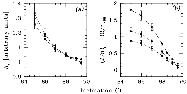
Fig. 12a and b. Importance of projection effects on the results obtained. An intrinsic axis ratio of (\frac{b}{a})_0 = 0.11 was assumed (Guthrie, 1992). Projection effects are shown for a vertical surface brightness profile at the galaxy center (short-dashed line), at 1 radial scale length (dotted line) and at 2 radial scale lengths (long-dashed line). a Projection effects cause an increasing scale height with increasing deviations from a 90^\circ inclination; b The influence of projection effects on the 2/n parameter.
