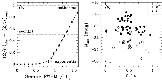
Fig. 8. a The influence of atmospheric smearing on an exponential vertical luminosity profile. The difference between the true and the observed distributions is shown as a function of the seeing FWHM, in units of the profile's scale height; b Distribution of absolute magnitude versus 2/n , the typical error size is indicated in the lower left corner.
