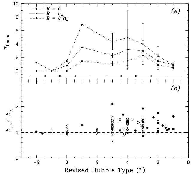
Fig. 11. a Maximum I -band optical depths as a function of galaxy type. The errors are statistical errors; where no error bars are given, only one data point was available in the specific type bin, indicated by the bars; b Type dependence of the I vs. K' scale length ratio. The filled circles are from the observations presented in this paper, the open circles from Peletier et al. (1994), and the crosses from Peletier & Balcells (1997).
