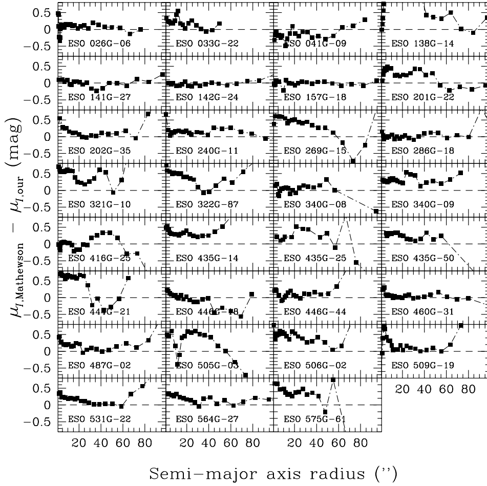
Fig. 3. Comparison between azimuthally averaged I -band profiles published by Mathewson et al. (1992) and Mathewson & Ford (1996), and those obtained from fitting ellipses to our observations.
