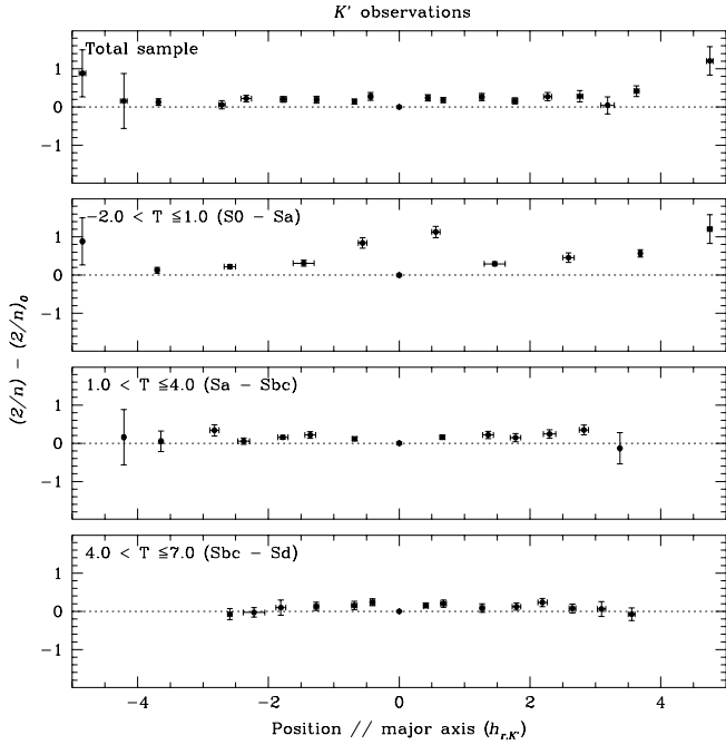
Fig. 7. Averaged distributions of the sharpness of the vertical profiles as a function of position along the major axis, both for the total K' -band sample and for specific bins in revised Hubble type, T .
