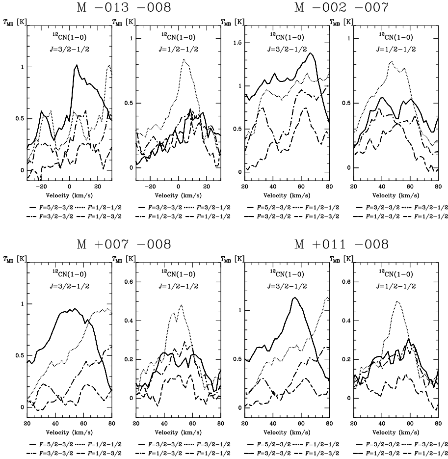
Fig. 3. Observed spectra of CN N=1-0 J=3/2-1/2 (left panel) and J=1/2-1/2 (right panel) toward the indicated clouds in the Galactic center region. All hyperfine components were obtained simultaneously in the same AOS backend; these profiles have been split and shifted by their frequency difference.
