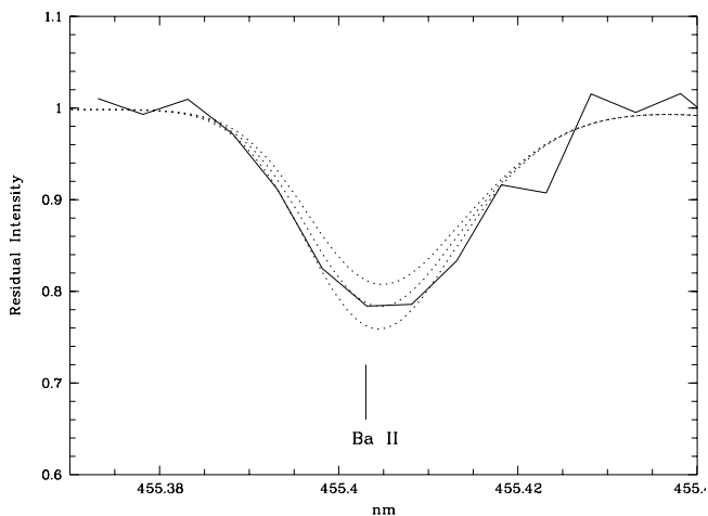
Fig. 4. The Ba II resonance line. The dotted lines are synthetic spectra with \epsilon_{\text{Ba}} = -2.00 , \epsilon_{\text{Ba}} = -2.10 , and \epsilon_{\text{Ba}} = -2.20
