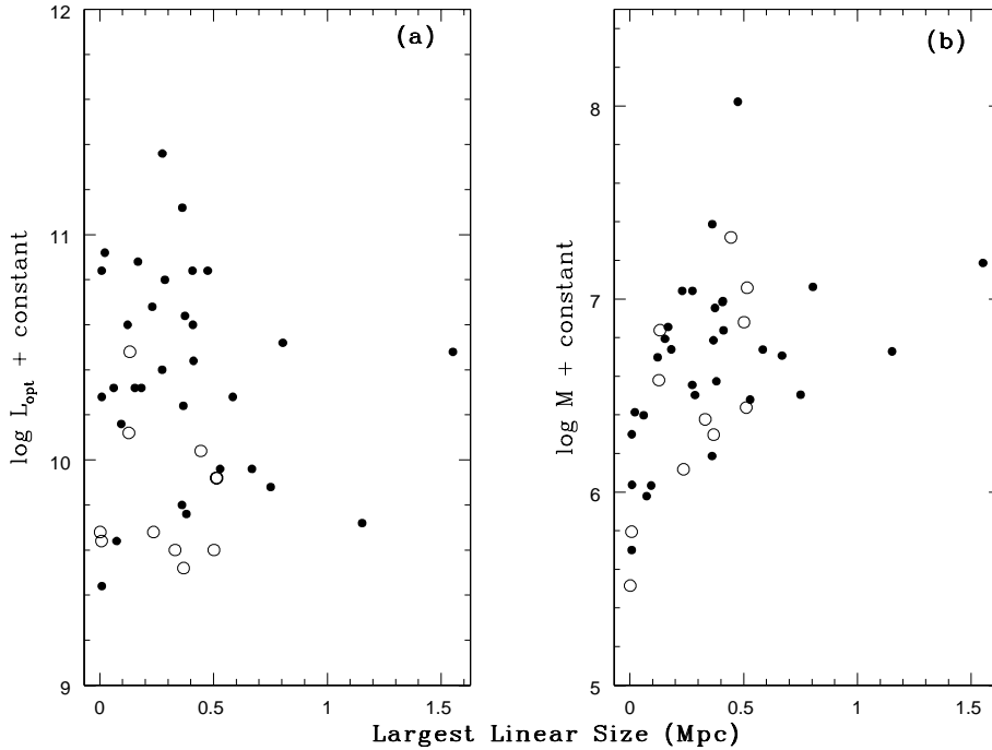
Fig. 2a and b. Plots of radio size ( l ) versus the optical luminosity and the mass of the central engine, respectively, for our combined dataset (see Sect. 4). The filled circle are the data from B(96) while the open circles refer to the data from JB(91), as explained in Sect. 2.
