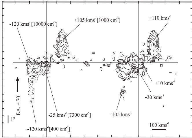
Fig. 2. A position-velocity diagram of LkH \alpha 233 in the region of the [SII] \lambda\lambda 6716/6731 lines. The slit has been oriented along the outflow axis as determined from Fig. 1. The velocities are relative to the stellar rest velocity (vertical lines), electron densities are indicated in square brackets ([ ]), and the spacing of the continuum levels is logarithmic, scaling by factors of 2^{1/2} . The horizontal line marks the centre of the continuum emission as determined from the fitting procedure (see Sect. 2).
