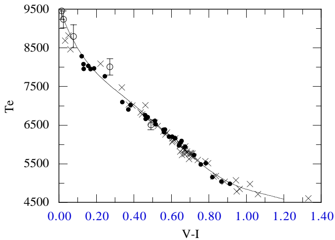
Fig. 2. Empirical T_{\text{eff}} versus V-I relation for dwarfs. Solid symbols are data from BLG94; crosses indicate AAM96 (for -0.2 < [\text{Fe}/\text{H}] < 0.2 ); open circles with error bars indicate Code et al. (1976)
