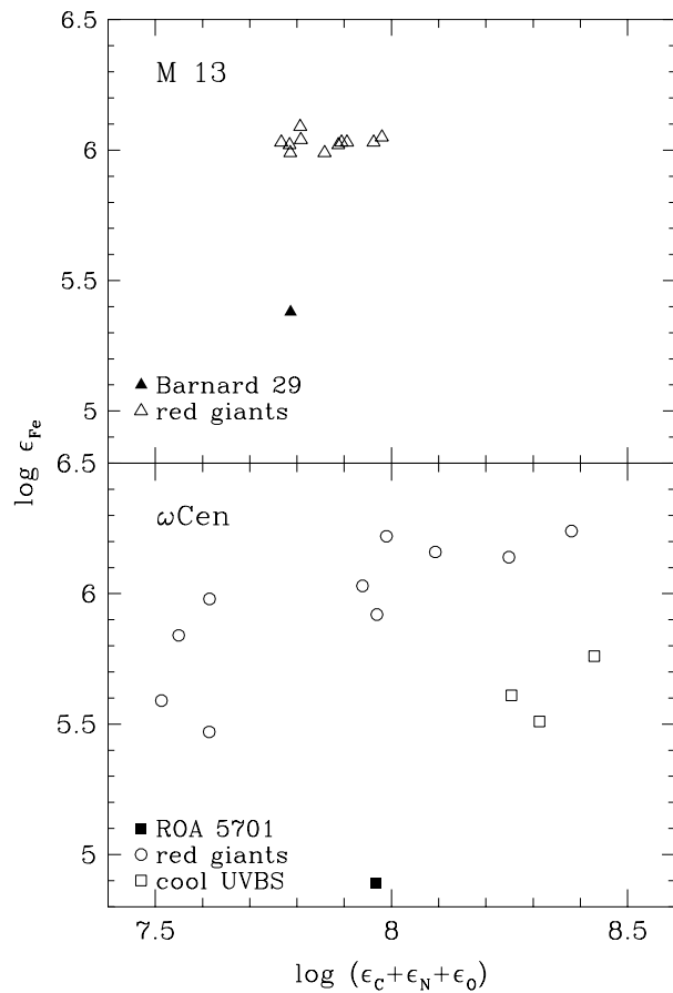
Fig. 4. Upper panel: The Fe abundances vs. the sum of CNO abundances for Barnard 29 compared to those of red giants in M 13. For references see text. Lower panel: The Fe abundances vs. the sum of CNO abundances for ROA 5701 compared to those of giants and cool UVBS in \omega Cen. For references see text.
