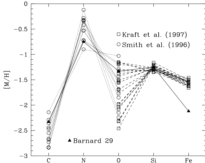
Fig. 2. The abundances derived for Barnard 29 compared to those of red giant stars in M 13. The solid line connects the abundances derived for Barnard 29 from curve-of-growth analyses. The dotted and short-dashed lines mark the abundances of the red giants taken from Smith et al. (1996) resp. Kraft et al. (1997).
