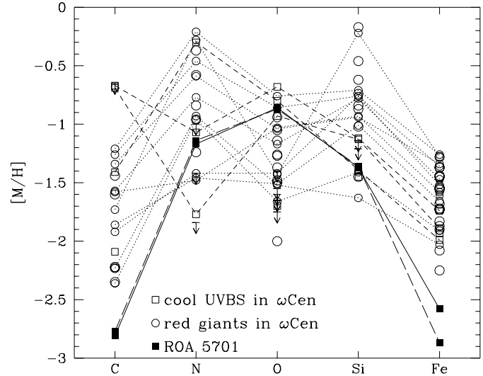
Fig. 3. The abundances derived for ROA 5701 compared to those of other stars in \omega Cen. The solid and long-dashed lines connect the abundances derived for ROA 5701 from curve-of-growth and spectrum synthesis analysis, respectively. The short dashed lines mark the cool UV bright stars, the dotted lines connect the abundances of the red giants. For references see text.
