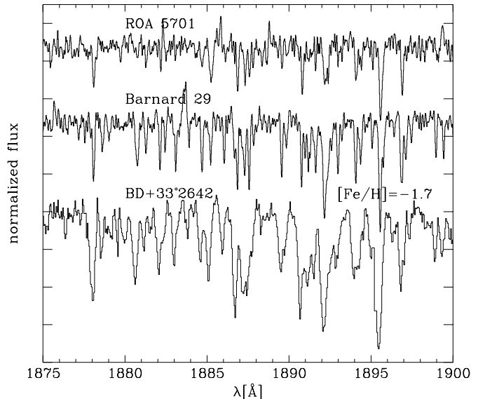
Fig. 1. The GHRS spectra of ROA 5701 and Barnard 29 , compared to IUE high resolution spectra of BD+33°2642 1 . The GHRS data were smoothed by convolution with a Gaussian of 0.06 Å FWHM, which yields a “smoothed” resolution of 0.09 Å, similar to that of the IUE data (0.1 Å). We used a microturbulent velocity of 10 km/s to derive the abundance noted for BD+33°2642.
