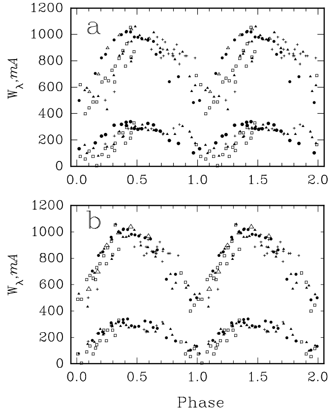
Fig. 3a and b. Spectroscopic variations vs. phases calculated with the linearly changing period (a) and with two constant periods (b) (see Fig. 3). W_{\lambda}(\text{Si II } 4128\text{-}31 \text{ and } 4201) are plotted; Table 1 data sets #4 and 6 (P1) are represented by filled triangles and open squares, respectively; and data sets #14 and 24 (P2) by open triangles and filled circles, respectively.
