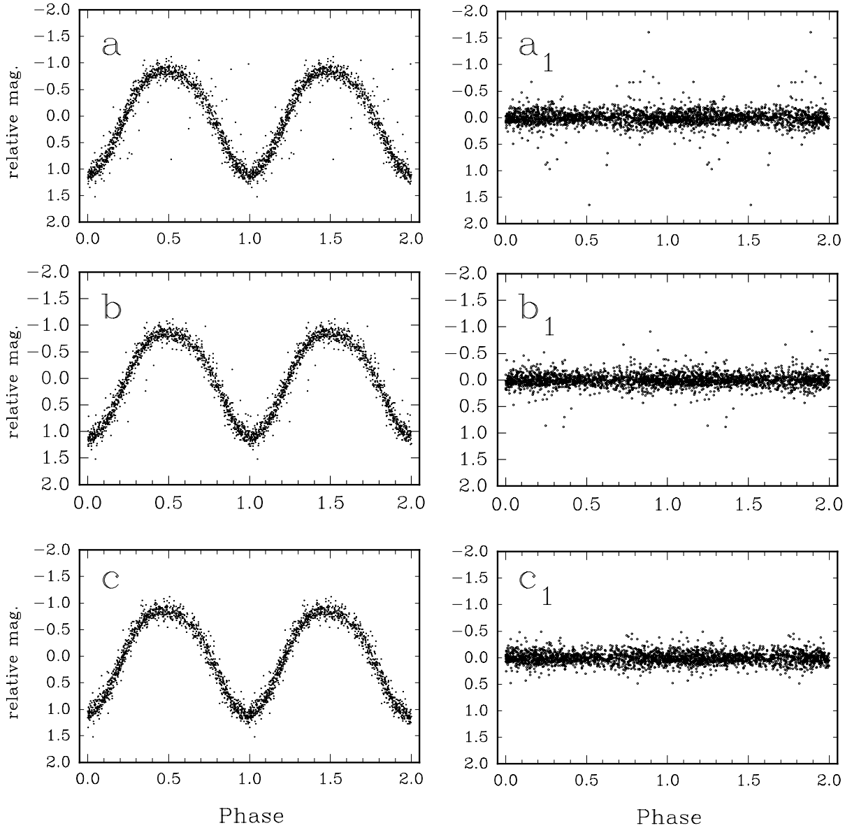
Fig. 2a–c1. Photometric variations vs. phases calculated with three different period approaches. a with a constant period 0^{\text{d}}.52070281 ; b with a linearly changing period (Sect. 3.1); and c with two periods constant periods P1=0^{\text{d}}.5206778 and P2=0^{\text{d}}.52070308 . In c , combined B+b ( b ) normalized magnitudes are from Table 1, data sets #1, 3, 5, 10, 11 (P1) and data sets #15, 16, 18–22, 25, 26 (P2). Right panels show the deviations from the mean curves.
