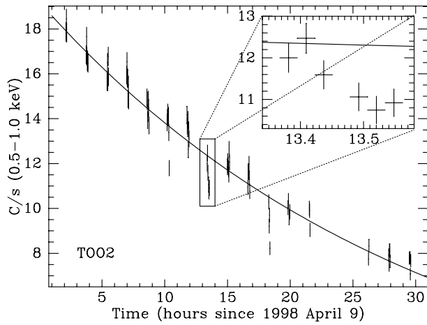
Fig. 3. 0.5–1.0 keV LECS light curve for TOO2 rebinned at 100 s, together with the exponential fit to the data ( \chi^2_\nu = 3.71 for 80 degrees of freedom). The inset shows an enlargement of the boxed data
