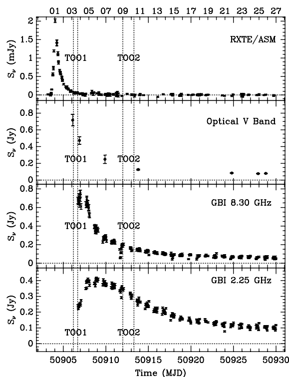
Fig. 1. Light curve of XTE J0421+560 in X-rays (2–12 keV), optical V, and radio (8.3 GHz and 2.25 GHz). Data come from the ASM (upper panel) and GBI (lower panels) public archives, IAU Circulars and our optical measurements (second panel). BeppoSAX observations are marked by dashed lines. The upper scale represents days of April 1998. ASM data after April 12 are upper limits
