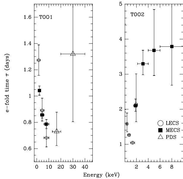
Fig. 2. Dependence of the e-folding time \tau on energy for the two BeppoSAX XTE J0421+560 observations
