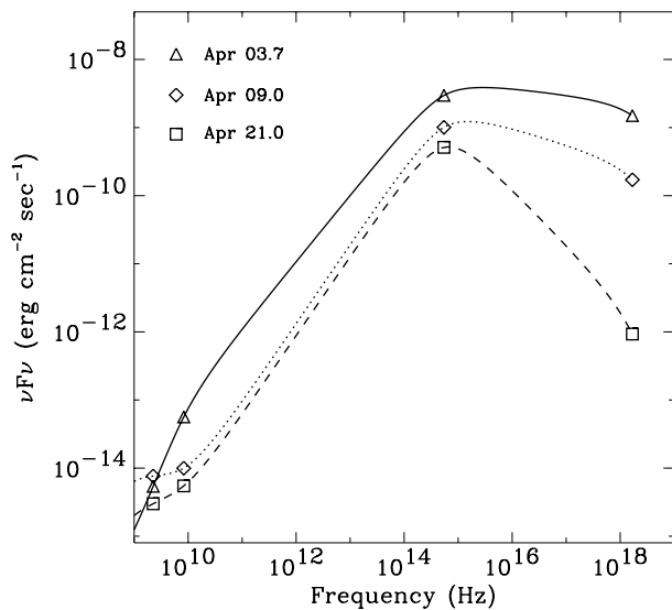
Fig. 4. \nu F\nu plot of XTE J0421+560 at different times during outburst. The lines are the interpolation with splines of the data points. The optical point is the average of B , V , R measurements. The Apr 21 X-ray point is estimated from the TOO2 decay law
