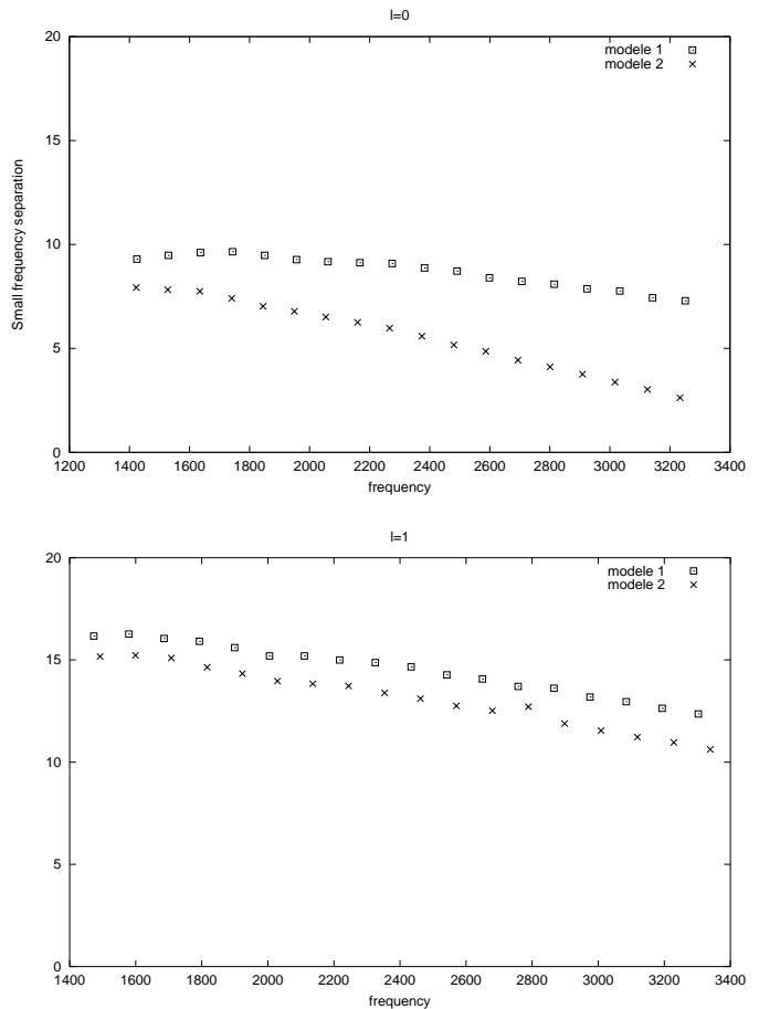
Fig. 3. \delta\nu ( l=0 ) as a function of \nu (in \mu\text{Hz} ) for Model 1 (squares) and Model 2 (crosses). The top panel is for l=0 and the bottom one for l=1
