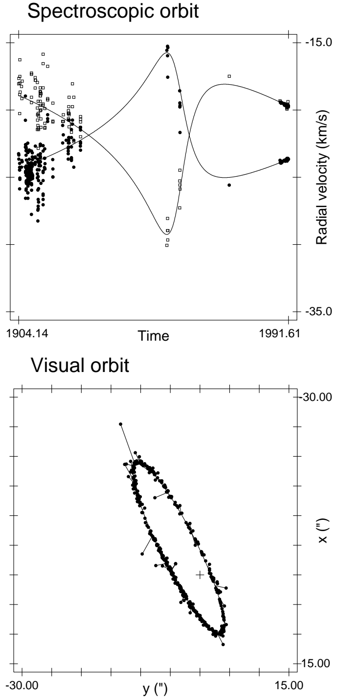
Fig. 1. Plot of the orbit corresponding to the best adjustment of all visual and spectroscopic data. The radial velocities of component B are represented with open squares. The radial velocities of Murdoch et al. (1993) are those after 1988
