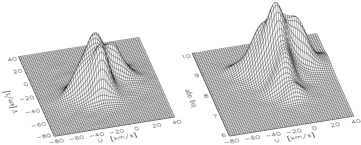
Fig. 3. (U,V) (left) and (U,log \tau ) (right) kernel density distribution of the total sample (in this plot h = h_{\text{gau}} in order to compare it with the field distribution in Fig. 5
