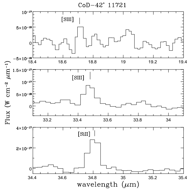
Fig. 3. Continuum subtracted SWS spectra of CoD-42 ^\circ 11721: selected ranges containing the [SIII] (18.7, 33.5 \mu\text{m} ) and [SiII] (34.8 \mu\text{m} ) lines.
