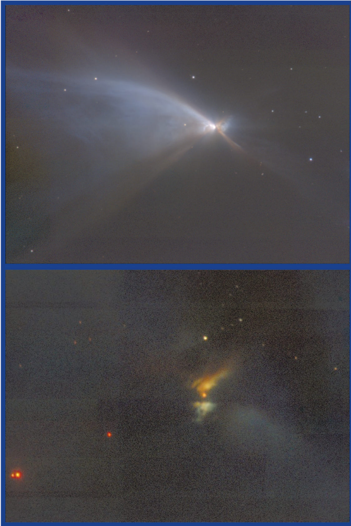
Fig. 1. VLT/UT1–ISAAC JHK observations of two young stellar objects in Chamaeleon. The objects are the Cha IR nebula (top) and Ced 110 IRS4 (bottom). North is up and east left in both images; the field sizes (in arcsec) are 166 \times 125 and 136 \times 100 , respectively
